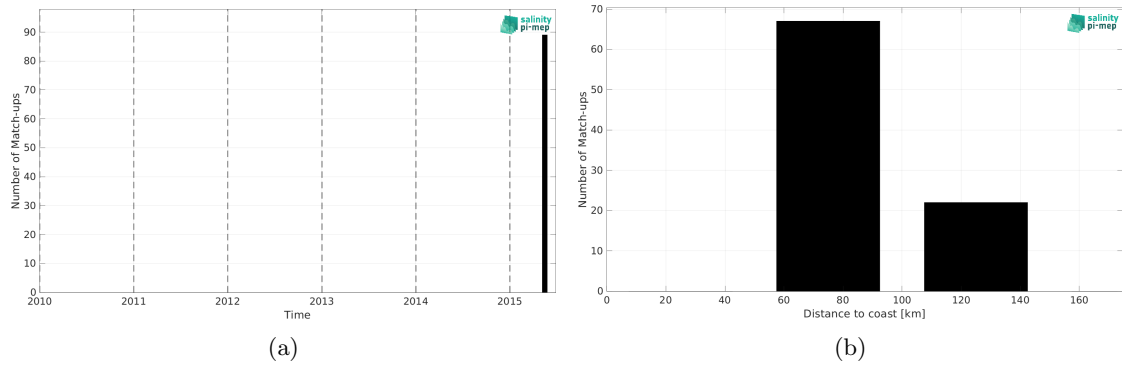
Figure 1: Number of match-ups between TSG (SAMOS) and Aquarius SSS L3 CAP v5 - 7-Day running (JPL) SSS as a function of time (a) and as function of the distance to coast (b) over the Ganga and Brahmaputra river plumes Pi-MEP region and for the full satellite product period.
