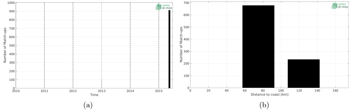
Figure 1: Number of match-ups between TSG (SAMOS) and Aquarius SSS L3 CAP v5 - 7-Day running (JPL) SSS as a function of time (a) and as function of the distance to coast (b) over the Ganga and Brahmaputra river plumes Pi-MEP region and for the full satellite product period.
