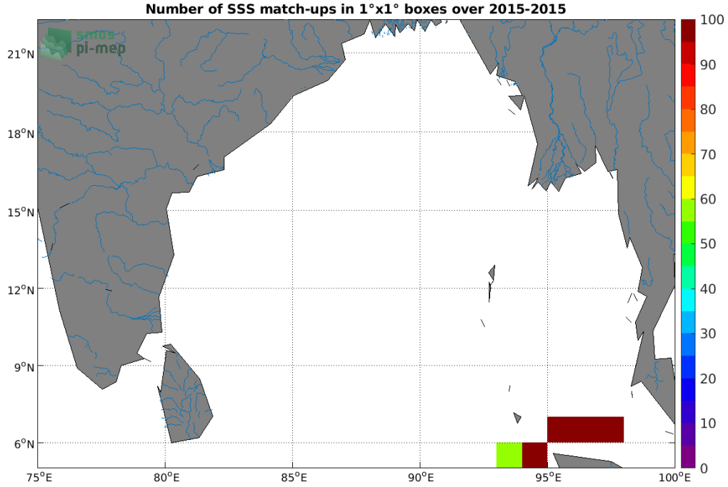
Figure 4: Number of SSS match-ups between TSG (SAMOS) SSS and the Aquarius SSS L3 CAP v5 - 7-Day running (JPL) SSS product for the Ganga and Brahmaputra river plumes Pi-MEP region over 1^\circ \times 1^\circ boxes and for the full satellite product period.
