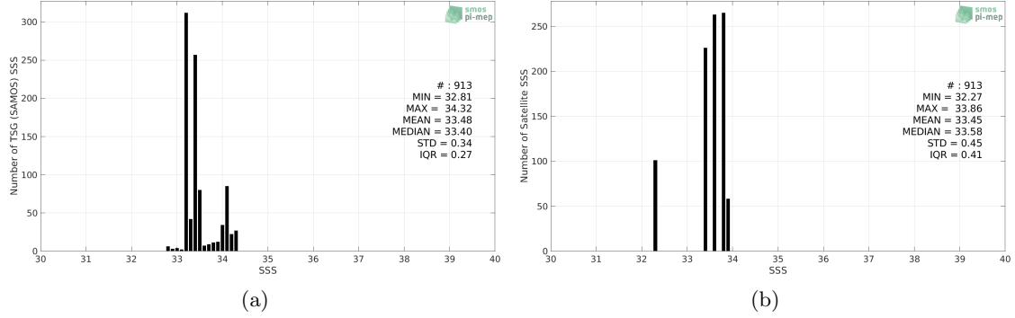
Figure 2: Histograms of SSS from TSG (SAMOS) (a) and Aquarius SSS L3 CAP v5 - 7-Day running (JPL) (b) considering all match-up pairs per bins of 0.1 over the Ganga and Brahmaputra river plumes Pi-MEP region and for the full satellite product period.
