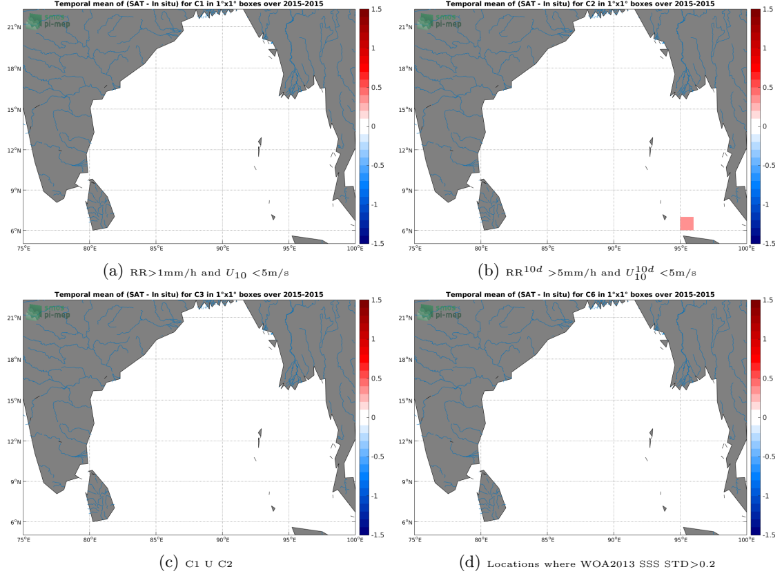
Figure 12: Temporal mean gridded over spatial boxes of size 1^\circ \times 1^\circ of \Delta SSS (Aquarius-L3-JPL-V5-7DAY-RUNNING - TSG-SAMOS) for 4 different subdatasets corresponding to: RR > 1\text{mm/h} and U_{10} < 5\text{m/s} (a), RR^{10d} > 5\text{mm/h} and U_{10}^{10d} < 5\text{m/s} (b), C1 U C2 (c), Locations where WOA2013 SSS STD > 0.2 (d).
