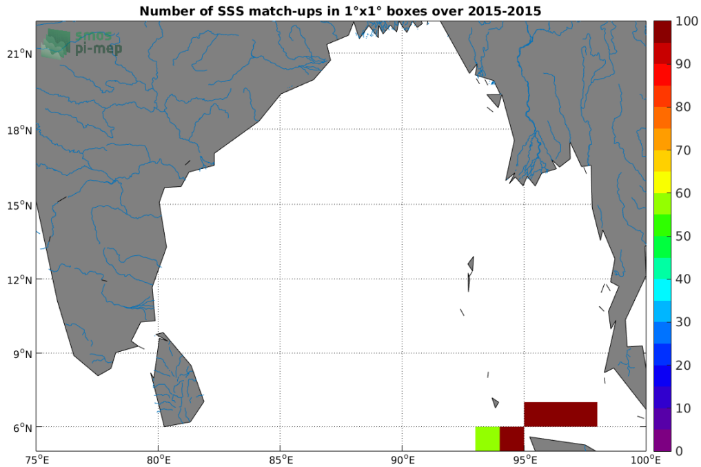
Figure 4: Number of SSS match-ups between TSG-SAMOS SSS and the Aquarius-L3-JPL-V5-7DAY-RUNNING SSS product for the Ganga and Brahmaputra river plumes Pi-MEP region over 1^\circ \times 1^\circ boxes and for the full satellite product period.
