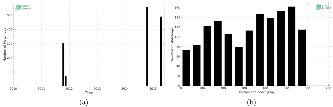
Figure 1: Number of match-ups between TSG-LEGOS-DM and Aquarius-L3-JPL-V5-7DAY-RUNNING SSS as a function of time (a) and as function of the distance to coast (b) over the Ganga and Brahmaputra river plumes Pi-MEP region and for the full satellite product period.
