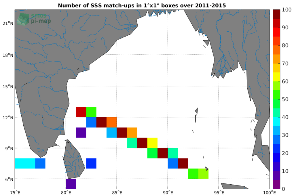
Figure 4: Number of SSS match-ups between TSG-LEGOS-DM SSS and the Aquarius-L3-JPL-V5-7DAY-RUNNING SSS product for the Ganga and Brahmaputra river plumes Pi-MEP region over 1^\circ \times 1^\circ boxes and for the full satellite product period.
