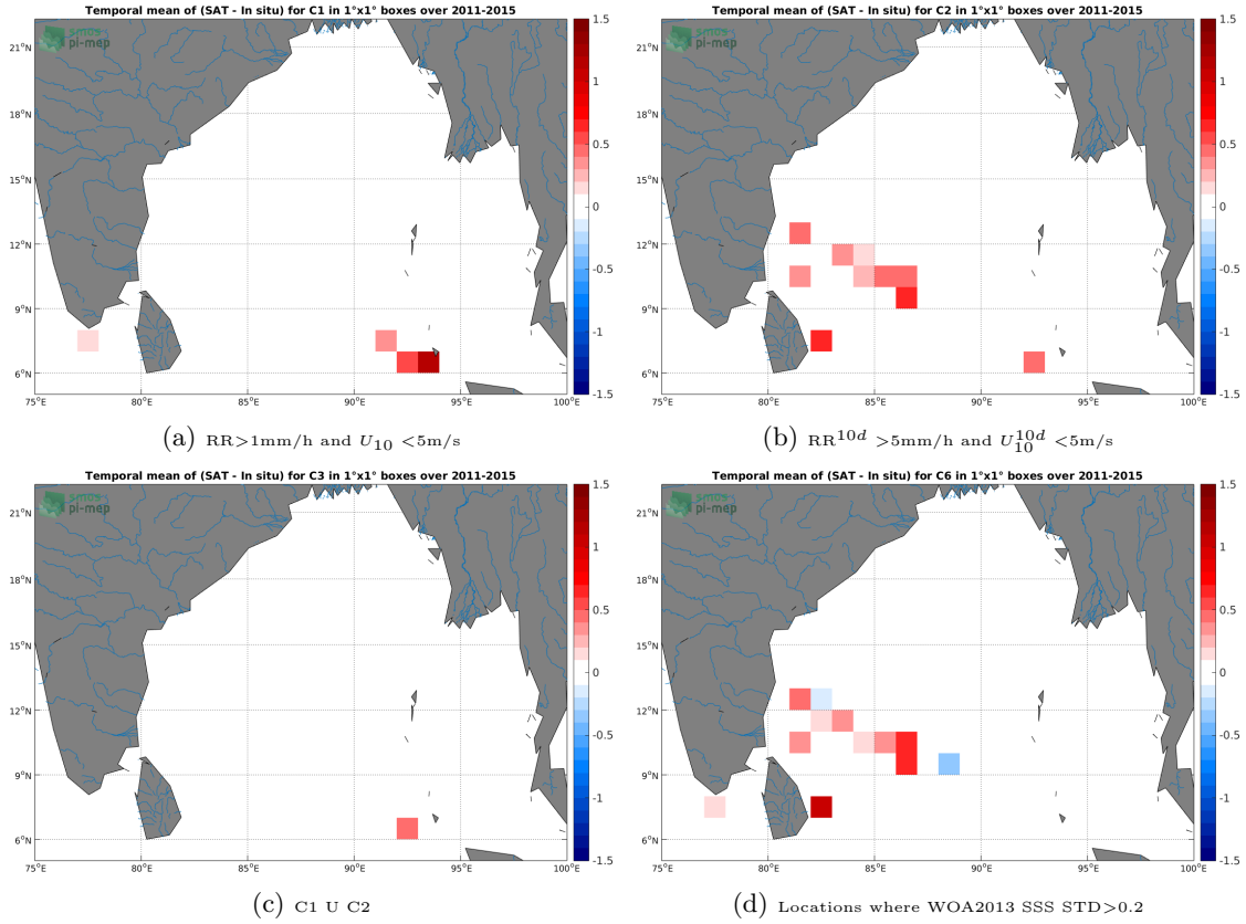
Figure 12: Temporal mean gridded over spatial boxes of size 1^\circ \times 1^\circ of \Delta SSS (Aquarius-L3-JPL-V5-7DAY-RUNNING - TSG-LEGOS-DM) for 4 different subdatasets corresponding to: RR > 1\text{mm/h} and U_{10} < 5\text{m/s} (a), RR^{10d} > 5\text{mm/h} and U_{10}^{10d} < 5\text{m/s} (b), C1 U C2 (c), Locations where WOA2013 SSS STD > 0.2 (d).
