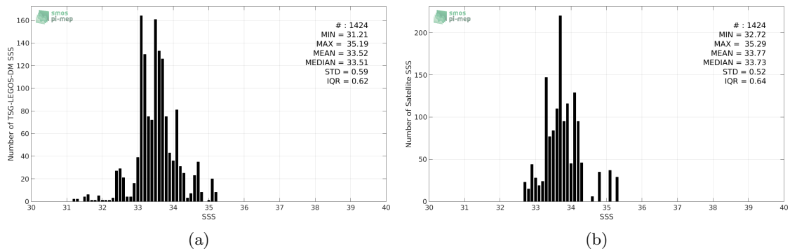
Figure 2: Histograms of SSS from TSG-LEGOS-DM (a) and Aquarius-L3-JPL-V5-7DAY-RUNNING (b) considering all match-up pairs per bins of 0.1 over the Ganga and Brahmaputra river plumes Pi-MEP region and for the full satellite product period.
