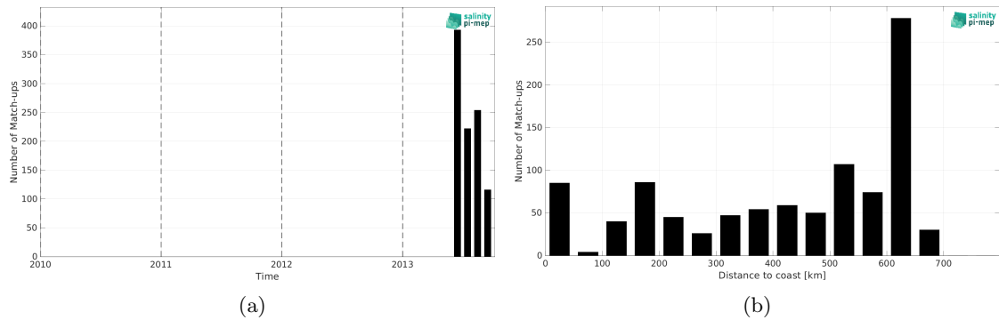
Figure 2: Number of match-ups between Surface drifters and Aquarius SSS L3 CAP v5 - 7-Day running (JPL) SSS as a function of time (a) and as function of the distance to coast (b) over the Ganga and Brahmaputra river plumes Pi-MEP region and for the full satellite product period.
