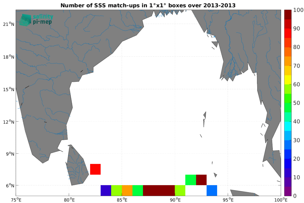
Figure 4: Number of SSS match-ups between Surface drifters SSS and the Aquarius SSS L3 CAP v5 - 7-Day running (JPL) SSS product for the Ganga and Brahmaputra river plumes Pi-MEP region over 1^\circ \times 1^\circ boxes and for the full satellite product period.
