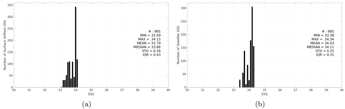
Figure 3: Histograms of SSS from Surface drifters (a) and Aquarius SSS L3 CAP v5 - 7-Day running (JPL) (b) considering all match-up pairs per bins of 0.1 over the Ganga and Brahmaputra river plumes Pi-MEP region and for the full satellite product period.
