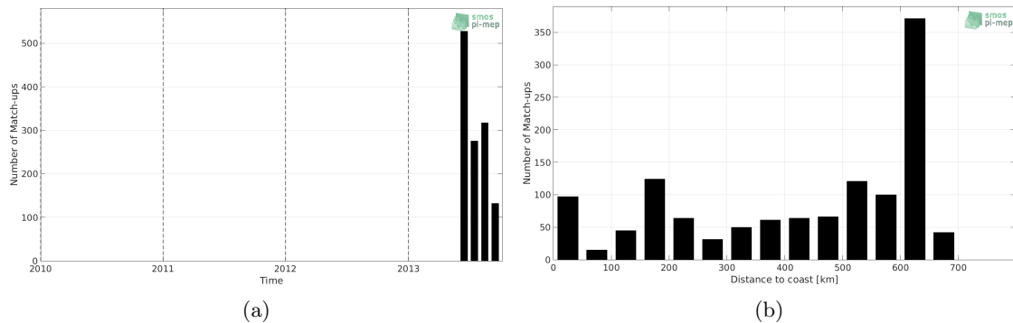
Figure 1: Number of match-ups between Surface drifters and Aquarius-L3-JPL-V5-7DAY-RUNNING SSS as a function of time (a) and as function of the distance to coast (b) over the Ganga and Brahmaputra river plumes Pi-MEP region and for the full satellite product period.
