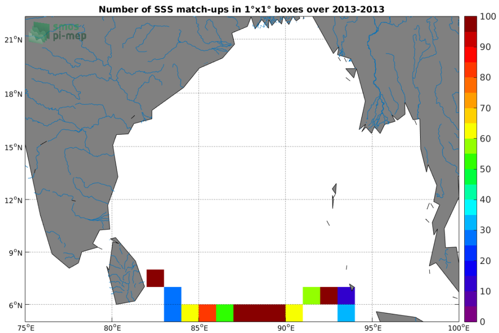
Figure 3: Number of SSS match-ups between Surface drifters SSS and the Aquarius-L3-JPL-V5-7DAY-RUNNING SSS product for the Ganga and Brahmaputra river plumes Pi-MEP region over 1°x1° boxes and for the full satellite product period.
