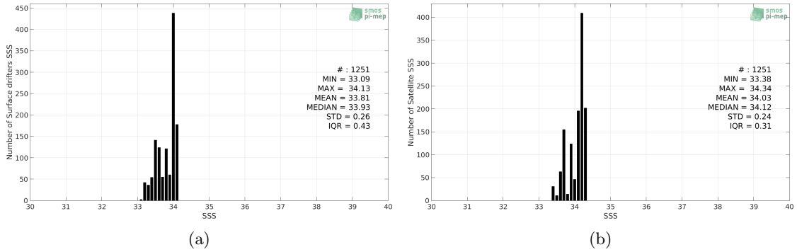
Figure 2: Histograms of SSS from Surface drifters (a) and Aquarius-L3-JPL-V5-7DAY-RUNNING (b) considering all match-up pairs per bins of 0.1 over the Ganga and Brahmaputra river plumes Pi-MEP region and for the full satellite product period.
