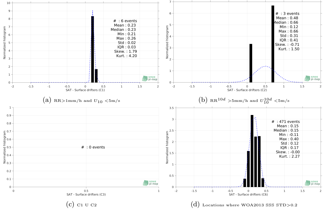
Figure 12: Normalized histogram of \Delta\text{SSS} (Aquarius-L3-JPL-V5-7DAY-RUNNING - Surface drifters) for 6 different subdatasets corresponding to: RR > 1mm/h and U_{10} < 5\text{m/s} (a), RR^{10d} > 5\text{mm/h} and U_{10}^{10d} < 5\text{m/s} (b), C1 U C2 (c), Locations where WOA2013 SSS STD > 0.2 (d).
