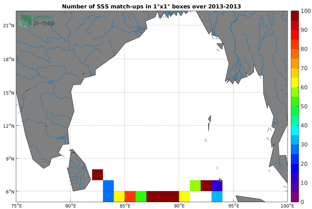
Figure 3: Number of SSS match-ups between Surface drifters SSS and the Aquarius-L3-JPL-V5-7DAY-RUNNING SSS product for the Ganga and Brahmaputra river plumes Pi-MEP region over 1^\circ \times 1^\circ boxes and for the full satellite product period.
