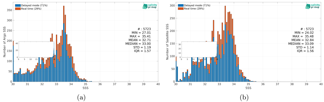
Figure 3: Histograms of SSS from Argo (a) and Aquarius SSS L3 CAP v5 - 7-Day running (JPL) (b) considering all match-up pairs per bins of 0.1 over the Ganga and Brahmaputra river plumes Pi-MEP region and for the full satellite product period.
