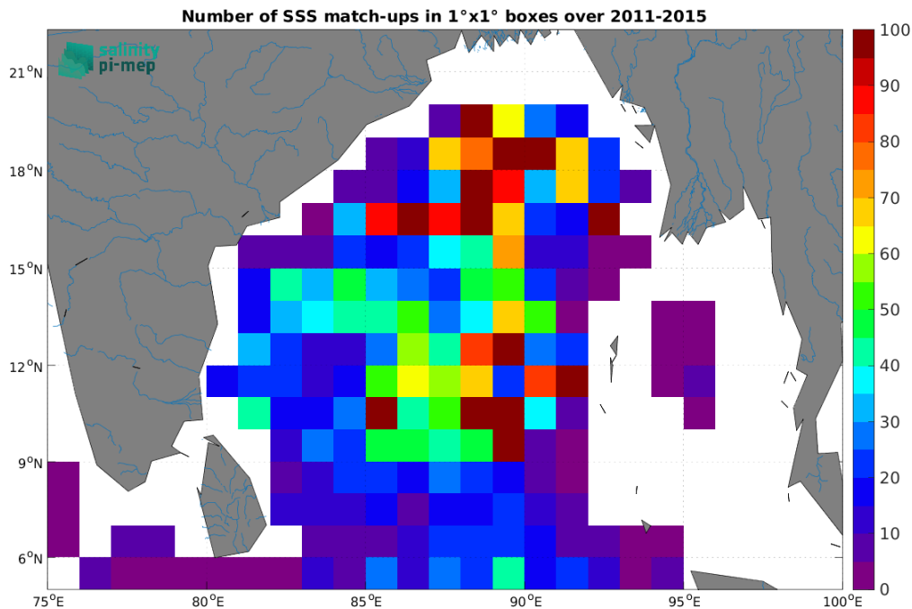
Figure 5: Number of SSS match-ups between Argo SSS and the Aquarius SSS L3 CAP v5 - 7-Day running (JPL) SSS product for the Ganga and Brahmaputra river plumes Pi-MEP region over 1^\circ \times 1^\circ boxes and for the full satellite product period.
