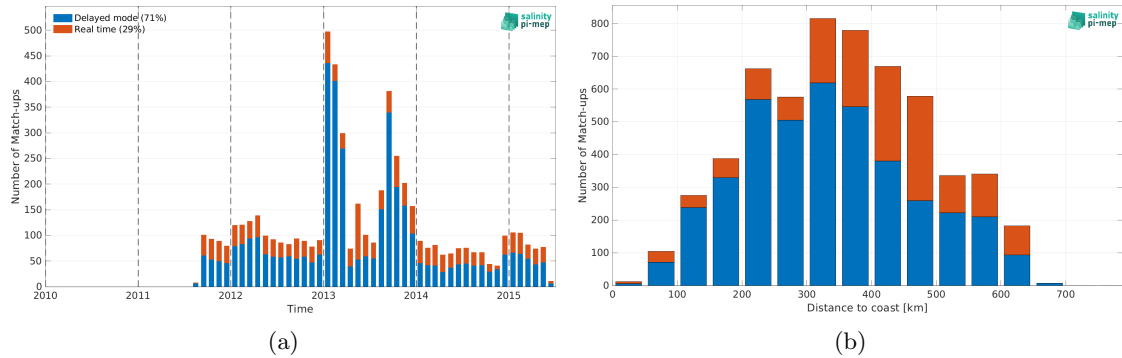
Figure 2: Number of match-ups between Argo and Aquarius SSS L3 CAP v5 - 7-Day running (JPL) SSS as a function of time (a) and as function of the distance to coast (b) over the Ganga and Brahmaputra river plumes Pi-MEP region and for the full satellite product period.
