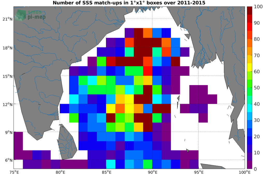
Figure 4: Number of SSS match-ups between Argo SSS and the Aquarius SSS L3 CAP v5 - 7-Day running (JPL) SSS product for the Ganga and Brahmaputra river plumes Pi-MEP region over 1^\circ \times 1^\circ boxes and for the full satellite product period.
