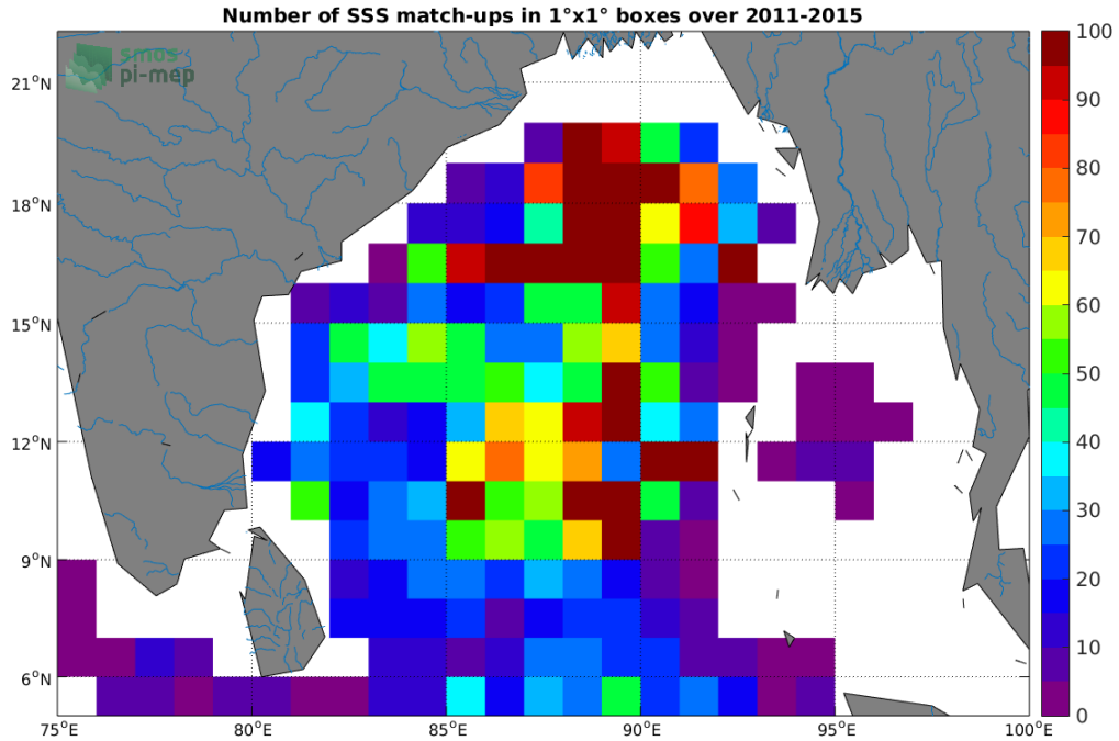
Figure 4: Number of SSS match-ups between Argo SSS and the Aquarius-L3-JPL-V5-7DAY-RUNNING SSS product for the Ganga and Brahmaputra river plumes Pi-MEP region over 1^\circ \times 1^\circ boxes and for the full satellite product period.
