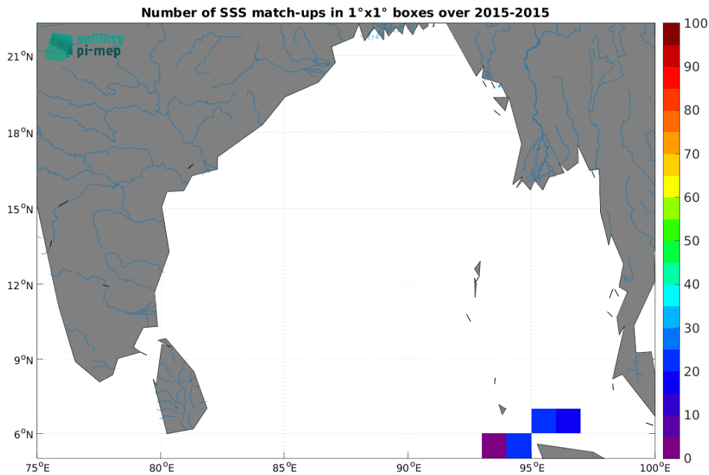
Figure 5: Number of SSS match-ups between TSG (SAMOS) SSS and the Aquarius SSS L3 CAP v5 - Monthly (JPL) SSS product for the Ganga and Brahmaputra river plumes Pi-MEP region over 1^\circ \times 1^\circ boxes and for the full satellite product period.
