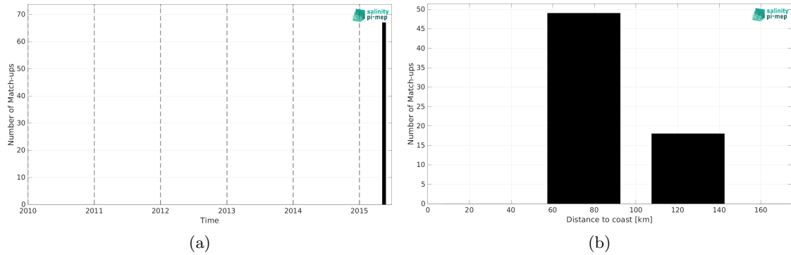
Figure 2: Number of match-ups between TSG (SAMOS) and Aquarius SSS L3 CAP v5 - Monthly (JPL) SSS as a function of time (a) and as function of the distance to coast (b) over the Ganga and Brahmaputra river plumes Pi-MEP region and for the full satellite product period.
