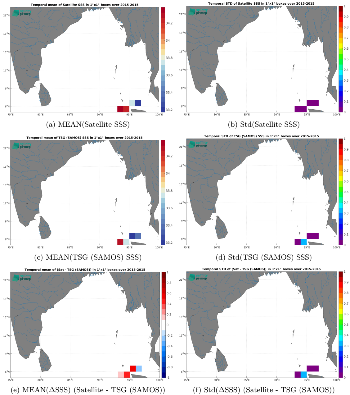
Figure 7: Temporal mean (left) and Std (right) of SSS from Aquarius SSS L3 CAP v5 - Monthly (JPL) (top), TSG (SAMOS) (middle), and of \Delta SSS (Satellite - TSG (SAMOS)). Only match-up pairs are used to generate these maps.
