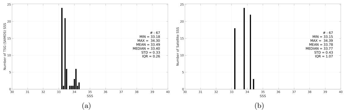
Figure 3: Histograms of SSS from TSG (SAMOS) (a) and Aquarius SSS L3 CAP v5 - Monthly (JPL) (b) considering all match-up pairs per bins of 0.1 over the Ganga and Brahmaputra river plumes Pi-MEP region and for the full satellite product period.
