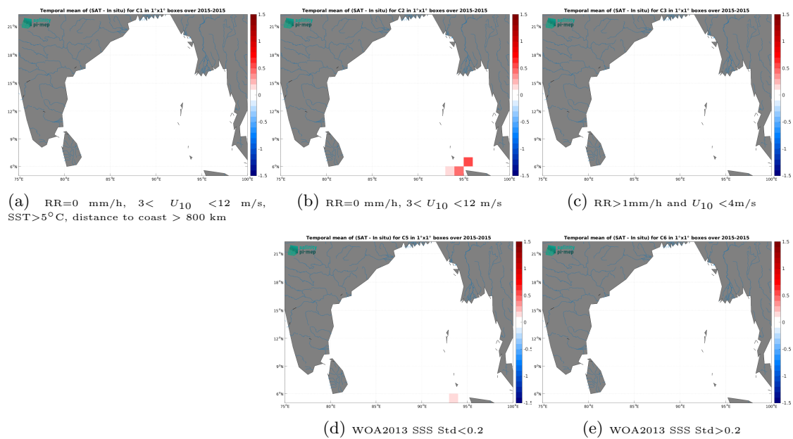
Figure 14: Temporal mean gridded over spatial boxes of size 1^\circ \times 1^\circ of \Delta SSS (Aquarius SSS L3 CAP v5 - Monthly (JPL) - TSG (SAMOS)) for 5 different subdatasets corresponding to:RR=0 mm/h, 3 < U_{10} < 12 m/s, SST >5^\circ C, distance to coast > 800 km (a), RR=0 mm/h, 3 < U_{10} < 12 m/s (b), RR >1 mm/h and U_{10} < 4 m/s (c), WOA2013 SSS Std <0.2 (d), WOA2013 SSS Std >0.2 (e).
