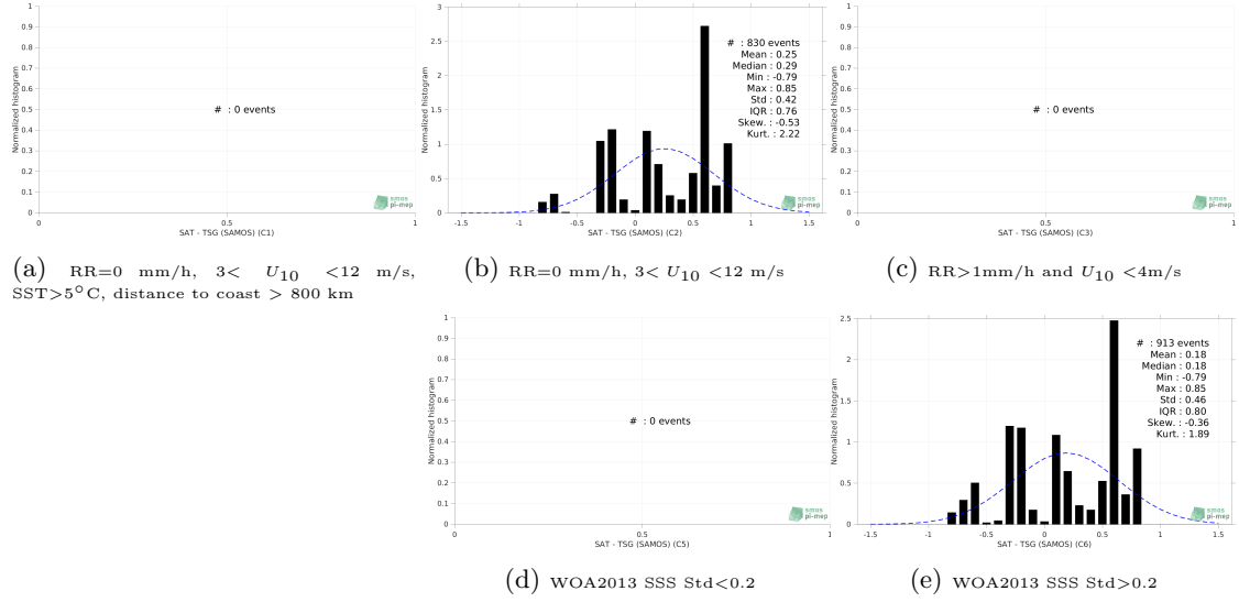
Figure 13: Normalized histogram of \Delta SSS (Aquarius SSS L3 CAP v5 - Monthly (JPL) - TSG (SAMOS)) for 5 different subdatasets corresponding to: RR=0 mm/h, 3 < U_{10} < 12 m/s, SST >5^{\circ} C, distance to coast > 800 km (a), RR=0 mm/h, 3 < U_{10} < 12 m/s (b), RR >1 mm/h and U_{10} < 4 m/s (c), WOA2013 SSS Std <0.2 (d), WOA2013 SSS Std >0.2 (e).
