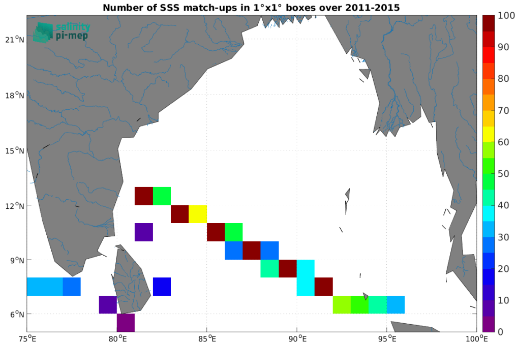
Figure 5: Number of SSS match-ups between TSG (LEGOS-DM) SSS and the Aquarius SSS L3 CAP v5 - Monthly (JPL) SSS product for the Ganga and Brahmaputra river plumes Pi-MEP region over 1^\circ \times 1^\circ boxes and for the full satellite product period.
