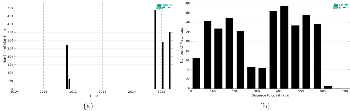
Figure 2: Number of match-ups between TSG (LEGOS-DM) and Aquarius SSS L3 CAP v5 - Monthly (JPL) SSS as a function of time (a) and as function of the distance to coast (b) over the Ganga and Brahmaputra river plumes Pi-MEP region and for the full satellite product period.
