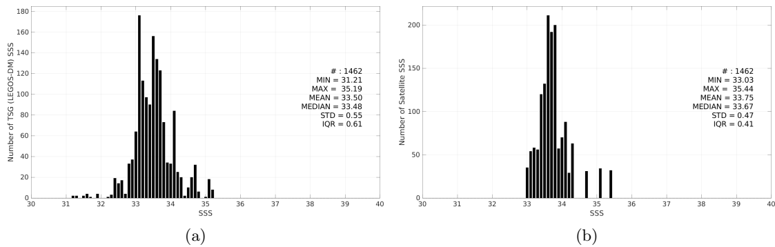
Figure 3: Histograms of SSS from TSG (LEGOS-DM) (a) and Aquarius SSS L3 CAP v5 - Monthly (JPL) (b) considering all match-up pairs per bins of 0.1 over the Ganga and Brahmaputra river plumes Pi-MEP region and for the full satellite product period.
