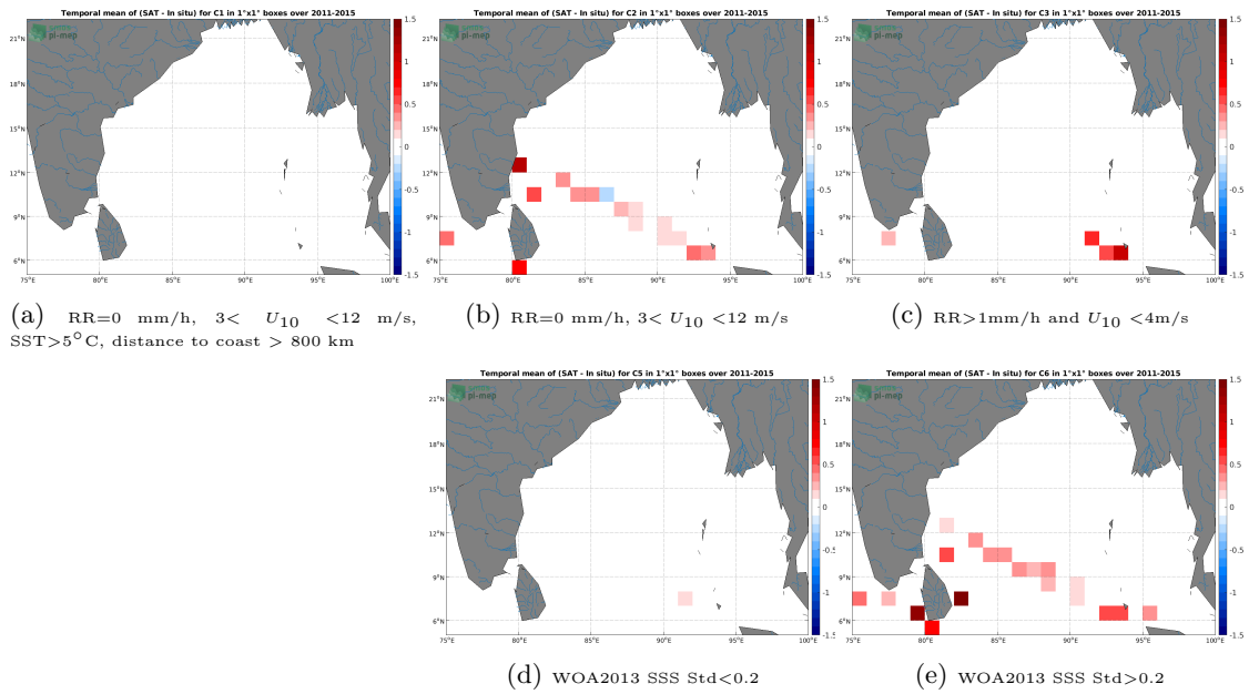
Figure 12: Temporal mean gridded over spatial boxes of size 1°x1° of \Delta SSS (Aquarius SSS L3 CAP v5 - Monthly (JPL) - TSG (LEGOS-DM)) for 5 different subdatasets corresponding to:RR=0 mm/h, 3 < U_{10} < 12 m/s, SST>5°C, distance to coast > 800 km (a), RR=0 mm/h, 3 < U_{10} < 12 m/s (b), RR>1mm/h and U_{10} < 4 m/s (c), WOA2013 SSS Std<0.2 (d), WOA2013 SSS Std>0.2 (e).
