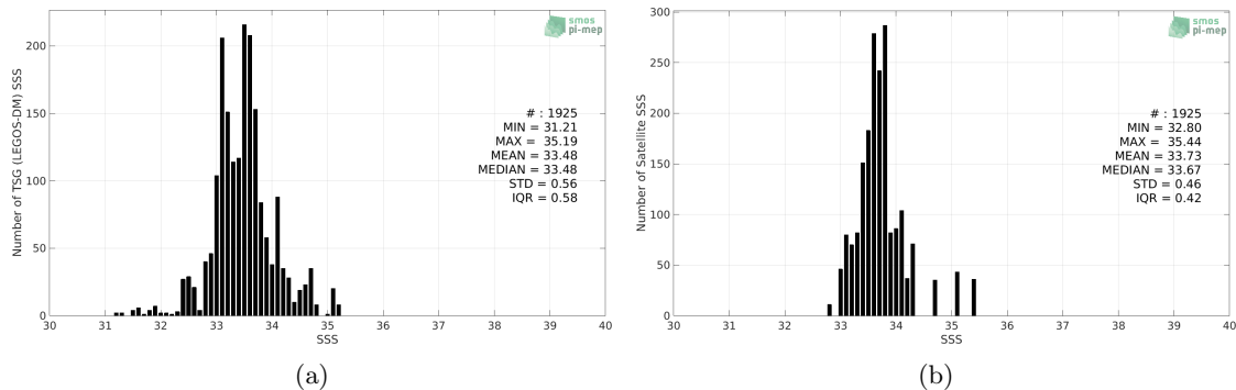
Figure 2: Histograms of SSS from TSG (LEGOS-DM) (a) and Aquarius SSS L3 CAP v5 - Monthly (JPL) (b) considering all match-up pairs per bins of 0.1 over the Ganga and Brahma-putra river plumes Pi-MEP region and for the full satellite product period.
