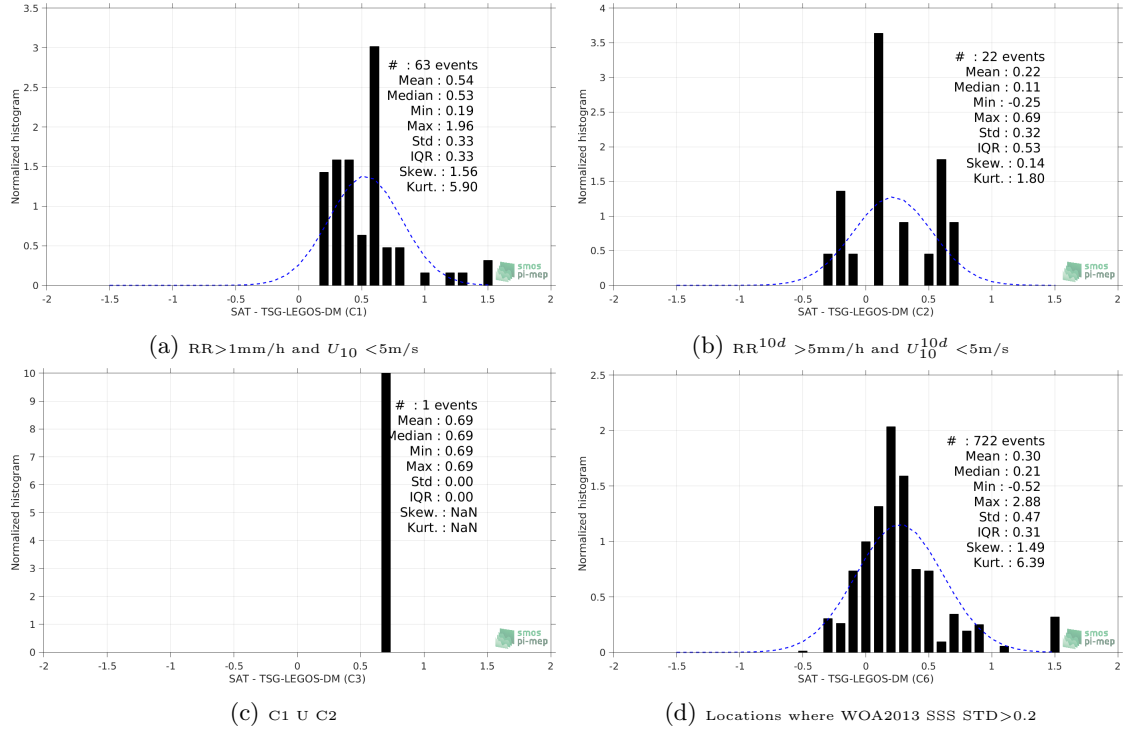
Figure 13: Normalized histogram of \Delta SSS (Aquarius-L3-JPL-V5-MONTHLY - TSG-LEGOS-DM) for 6 different subdatasets corresponding to: RR > 1mm/h and U_{10} < 5 m/s (a), RR^{10d} > 5 mm/h and U_{10}^{10d} < 5 m/s (b), C1 U C2 (c), Locations where WOA2013 SSS STD > 0.2 (d).
