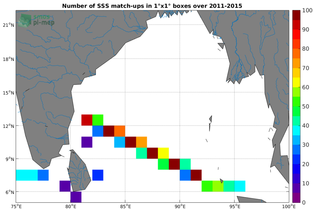
Figure 4: Number of SSS match-ups between TSG-LEGOS-DM SSS and the Aquarius-L3-JPL-V5-MONTHLY SSS product for the Ganga and Brahmaputra river plumes Pi-MEP region over 1°x1° boxes and for the full satellite product period.
