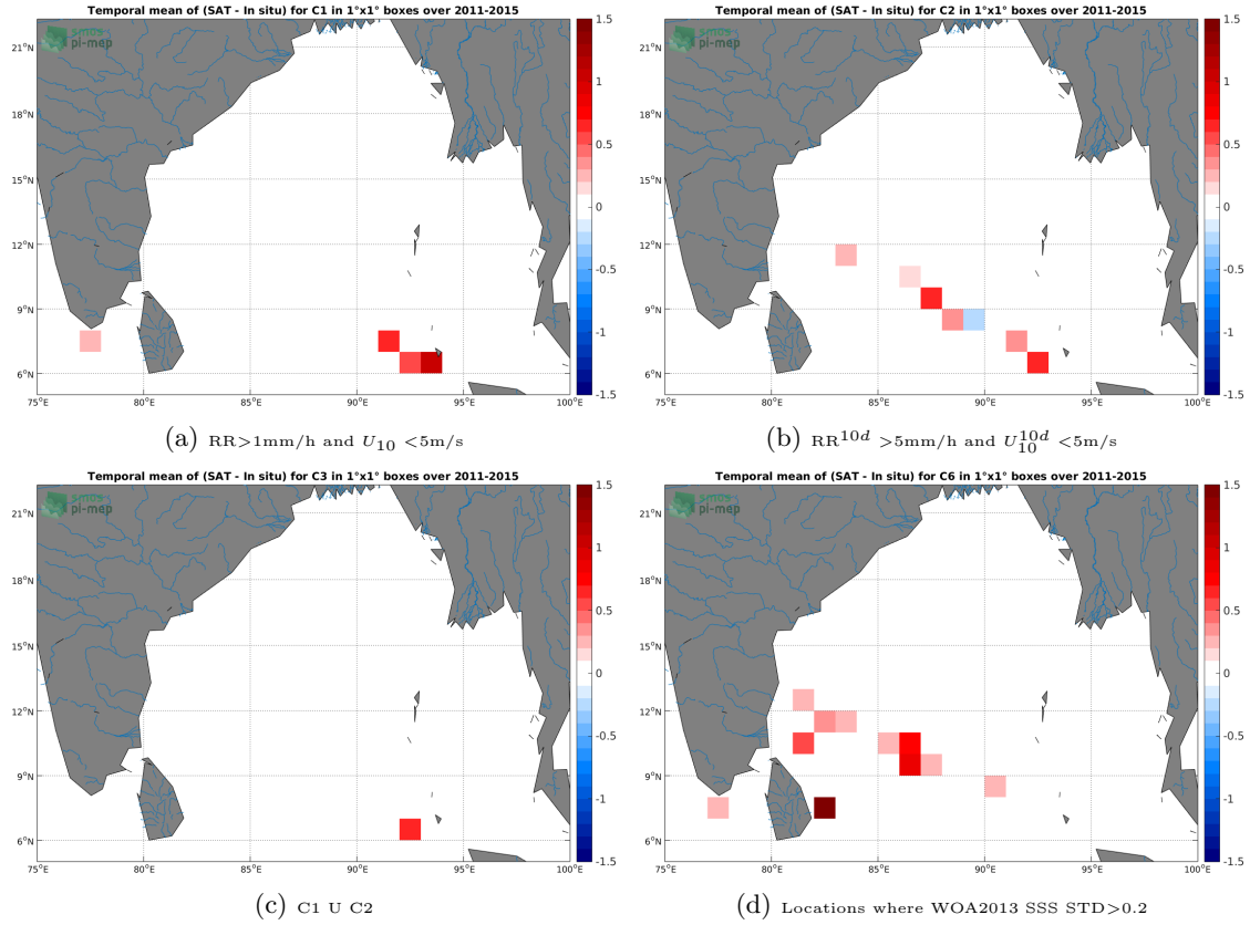
Figure 12: Temporal mean gridded over spatial boxes of size 1^\circ \times 1^\circ of \Delta SSS (Aquarius-L3-JPL-V5-MONTHLY - TSG-LEGOS-DM) for 4 different subdatasets corresponding to: RR > 1\text{mm/h} and U_{10} < 5\text{m/s} (a), RR^{10d} > 5\text{mm/h} and U_{10}^{10d} < 5\text{m/s} (b), C1 U C2 (c), Locations where WOA2013 SSS STD > 0.2 (d).
