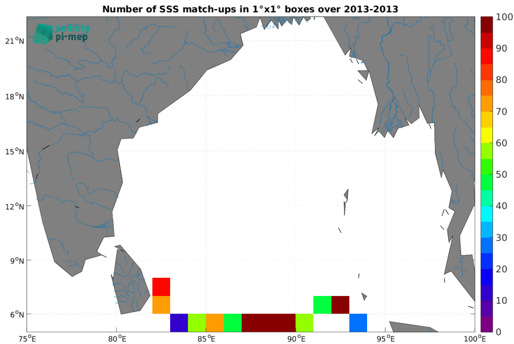
Figure 4: Number of SSS match-ups between Surface drifters SSS and the Aquarius SSS L3 CAP v5 - Monthly (JPL) SSS product for the Ganga and Brahmaputra river plumes Pi-MEP region over 1°×1° boxes and for the full satellite product period.
