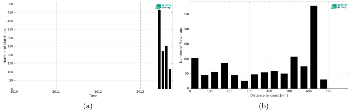
Figure 2: Number of match-ups between Surface drifters and Aquarius SSS L3 CAP v5 - Monthly (JPL) SSS as a function of time (a) and as function of the distance to coast (b) over the Ganga and Brahmaputra river plumes Pi-MEP region and for the full satellite product period.
