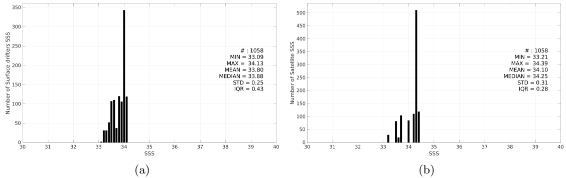
Figure 3: Histograms of SSS from Surface drifters (a) and Aquarius SSS L3 CAP v5 - Monthly (JPL) (b) considering all match-up pairs per bins of 0.1 over the Ganga and Brahmaputra river plumes Pi-MEP region and for the full satellite product period.
