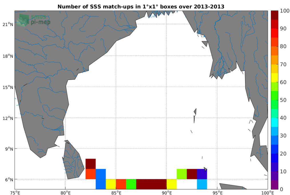
Figure 3: Number of SSS match-ups between Surface drifters SSS and the Aquarius-L3-JPL-V5-MONTHLY SSS product for the Ganga and Brahmaputra river plumes Pi-MEP region over 1^{\circ} \times 1^{\circ} boxes and for the full satellite product period.
