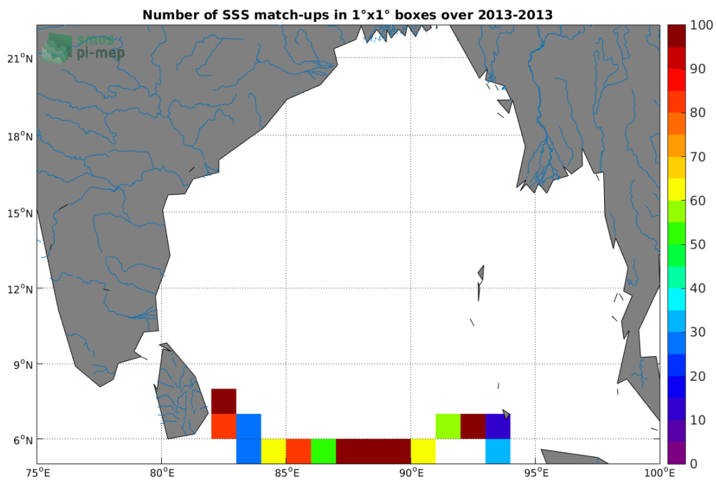
Figure 3: Number of SSS match-ups between Surface drifters SSS and the Aquarius-L3-JPL-V5-MONTHLY SSS product for the Ganga and Brahmaputra river plumes Pi-MEP region over 1^\circ \times 1^\circ boxes and for the full satellite product period.
