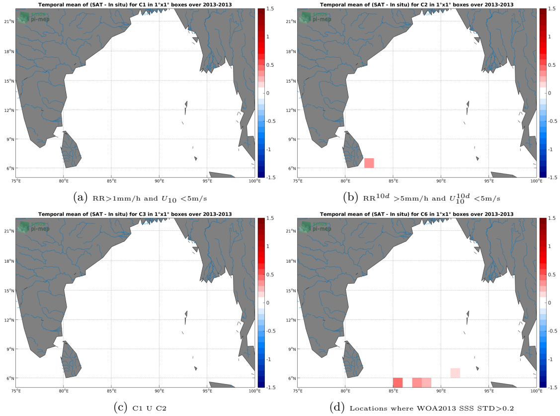
Figure 11: Temporal mean gridded over spatial boxes of size 1^\circ \times 1^\circ of \Delta SSS (Aquarius-L3-JPL-V5-MONTHLY - Surface drifters) for 4 different subdatasets corresponding to: RR > 1\text{mm/h} and U_{10} < 5\text{m/s} (a), RR^{10d} > 5\text{mm/h} and U_{10}^{10d} < 5\text{m/s} (b), C1 U C2 (c), Locations where WOA2013 SSS STD > 0.2 (d).
