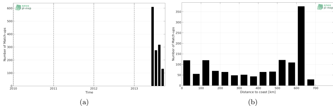
Figure 1: Number of match-ups between Surface drifters and Aquarius-L3-JPL-V5-MONTHLY SSS as a function of time (a) and as function of the distance to coast (b) over the Ganga and Brahmaputra river plumes Pi-MEP region and for the full satellite product period.
