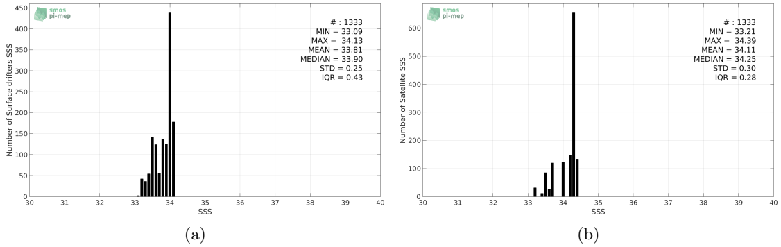
Figure 2: Histograms of SSS from Surface drifters (a) and Aquarius-L3-JPL-V5-MONTHLY (b) considering all match-up pairs per bins of 0.1 over the Ganga and Brahmaputra river plumes Pi-MEP region and for the full satellite product period.
