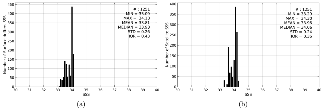
Figure 2: Histograms of SSS from Surface drifters (a) and Aquarius-L3-JPL-V4-7DAY-RUNNING (b) considering all match-up pairs per bins of 0.1 over the Ganga and Brahmaputra river plumes Pi-MEP region and for the full satellite product period.
