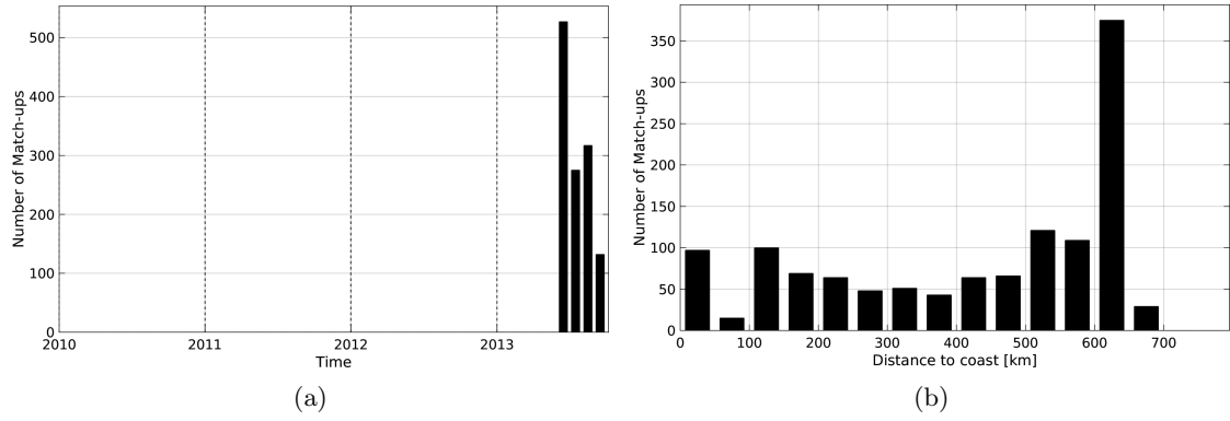
Figure 1: Number of match-ups between Surface drifters and Aquarius-L3-JPL-V4-7DAY-RUNNING SSS as a function of time (a) and as function of the distance to coast (b) over the Ganga and Brahmaputra river plumes Pi-MEP region and for the full satellite product period.
