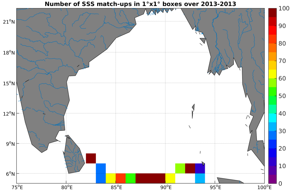
Figure 3: Number of SSS match-ups between Surface drifters SSS and the Aquarius-L3-JPL-V4-7DAY-RUNNING SSS product for the Ganga and Brahmaputra river plumes Pi-MEP region over 1^\circ \times 1^\circ boxes and for the full satellite product period.
