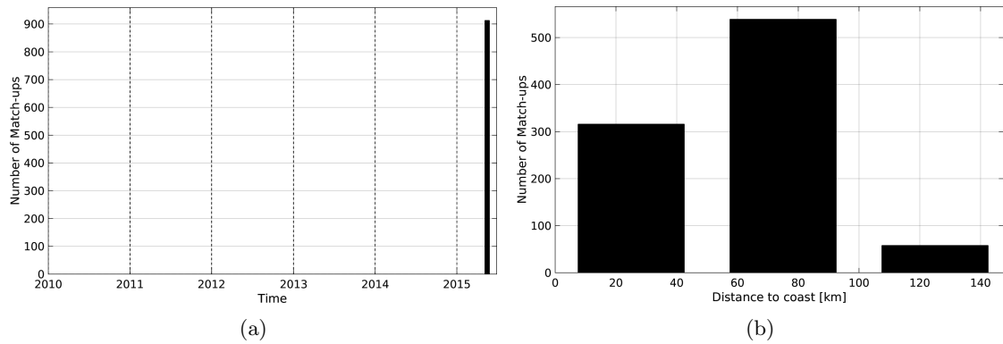
Figure 1: Number of match-ups between TSG-SAMOS and Aquarius-L3-JPL-V4-MONTHLY SSS as a function of time (a) and as function of the distance to coast (b) over the Ganga and Brahmaputra river plumes Pi-MEP region and for the full satellite product period.
