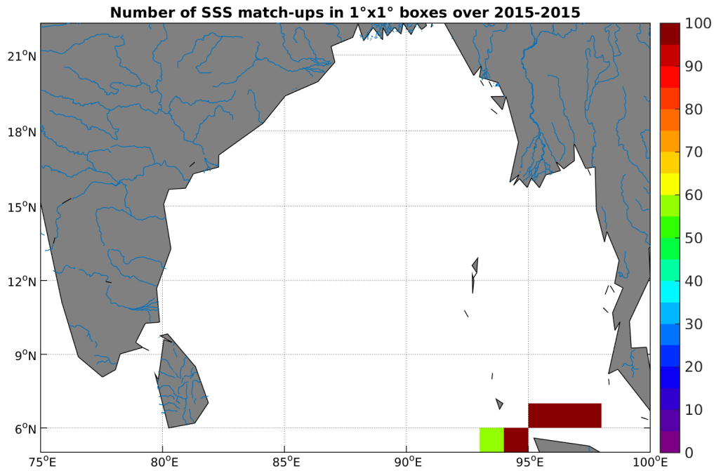
Figure 4: Number of SSS match-ups between TSG-SAMOS SSS and the Aquarius-L3-JPL-V4-MONTHLY SSS product for the Ganga and Brahmaputra river plumes Pi-MEP region over 1^\circ \times 1^\circ boxes and for the full satellite product period.
