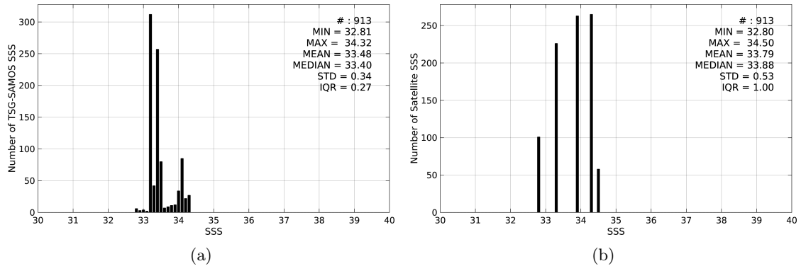
Figure 2: Histograms of SSS from TSG-SAMOS (a) and Aquarius-L3-JPL-V4-MONTHLY (b) considering all match-up pairs per bins of 0.1 over the Ganga and Brahmaputra river plumes Pi-MEP region and for the full satellite product period.
