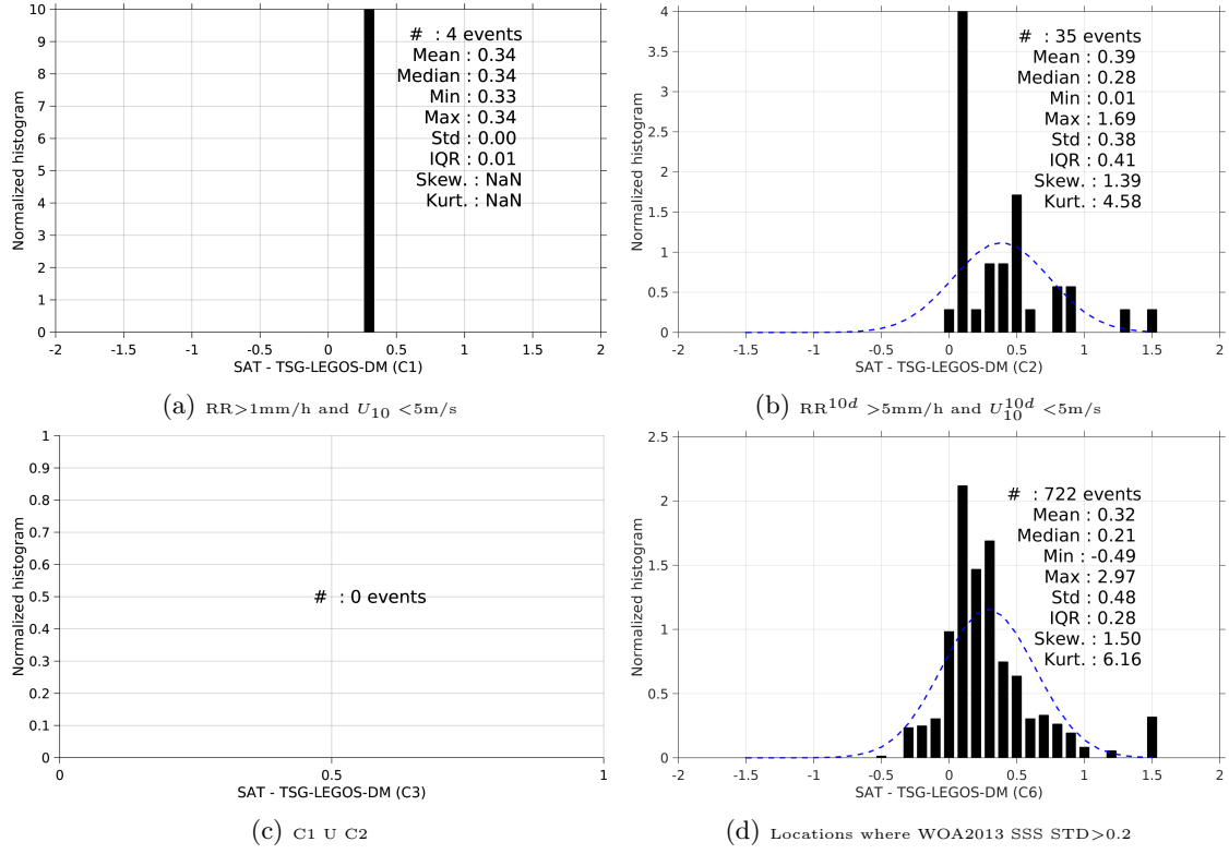
Figure 13: Normalized histogram of \Delta\text{SSS} (Aquarius-L3-JPL-V4-MONTHLY - TSG-LEGOS-DM) for 6 different subdatasets corresponding to: RR > 1\text{mm/h} and U_{10} < 5\text{m/s} (a), RR^{10d} > 5\text{mm/h} and U_{10}^{10d} < 5\text{m/s} (b), C1 \cup C2 (c), Locations where WOA2013 SSS STD > 0.2 (d).
