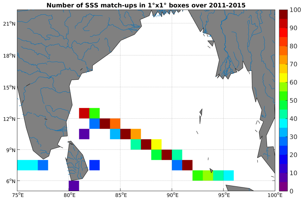
Figure 4: Number of SSS match-ups between TSG-LEGOS-DM SSS and the Aquarius-L3-JPL-V4-MONTHLY SSS product for the Ganga and Brahmaputra river plumes Pi-MEP region over 1^\circ \times 1^\circ boxes and for the full satellite product period.
