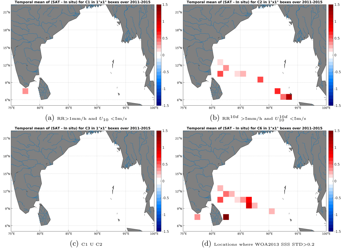
Figure 12: Temporal mean gridded over spatial boxes of size 1^\circ \times 1^\circ of \Delta SSS (Aquarius-L3-JPL-V4-MONTHLY - TSG-LEGOS-DM) for 4 different subdatasets corresponding to: RR > 1\text{mm/h} and U_{10} < 5\text{m/s} (a), RR^{10d} > 5\text{mm/h} and U_{10}^{10d} < 5\text{m/s} (b), C1 U C2 (c), Locations where WOA2013 SSS STD > 0.2 (d).
