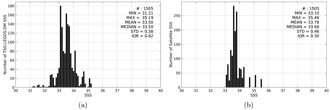
Figure 2: Histograms of SSS from TSG-LEGOS-DM (a) and Aquarius-L3-JPL-V4-MONTHLY (b) considering all match-up pairs per bins of 0.1 over the Ganga and Brahmaputra river plumes Pi-MEP region and for the full satellite product period.
