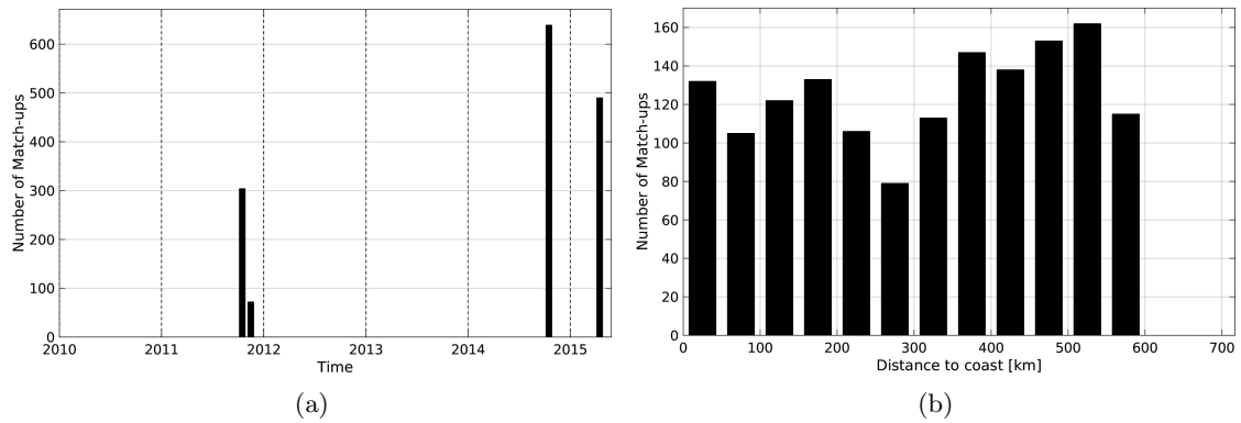
Figure 1: Number of match-ups between TSG-LEGOS-DM and Aquarius-L3-JPL-V4-MONTHLY SSS as a function of time (a) and as function of the distance to coast (b) over the Ganga and Brahmaputra river plumes Pi-MEP region and for the full satellite product period.
