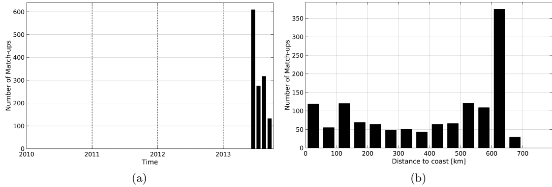
Figure 1: Number of match-ups between Surface drifters and Aquarius-L3-JPL-V4-MONTHLY SSS as a function of time (a) and as function of the distance to coast (b) over the Ganga and Brahmaputra river plumes Pi-MEP region and for the full satellite product period.
