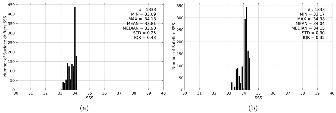
Figure 2: Histograms of SSS from Surface drifters (a) and Aquarius-L3-JPL-V4-MONTHLY (b) considering all match-up pairs per bins of 0.1 over the Ganga and Brahmaputra river plumes Pi-MEP region and for the full satellite product period.
