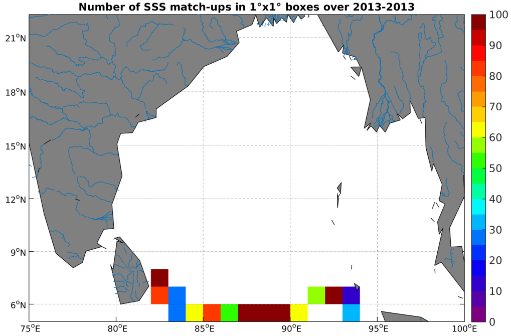
Figure 3: Number of SSS match-ups between Surface drifters SSS and the Aquarius-L3-JPL-V4-MONTHLY SSS product for the Ganga and Brahmaputra river plumes Pi-MEP region over 1°x1° boxes and for the full satellite product period.
