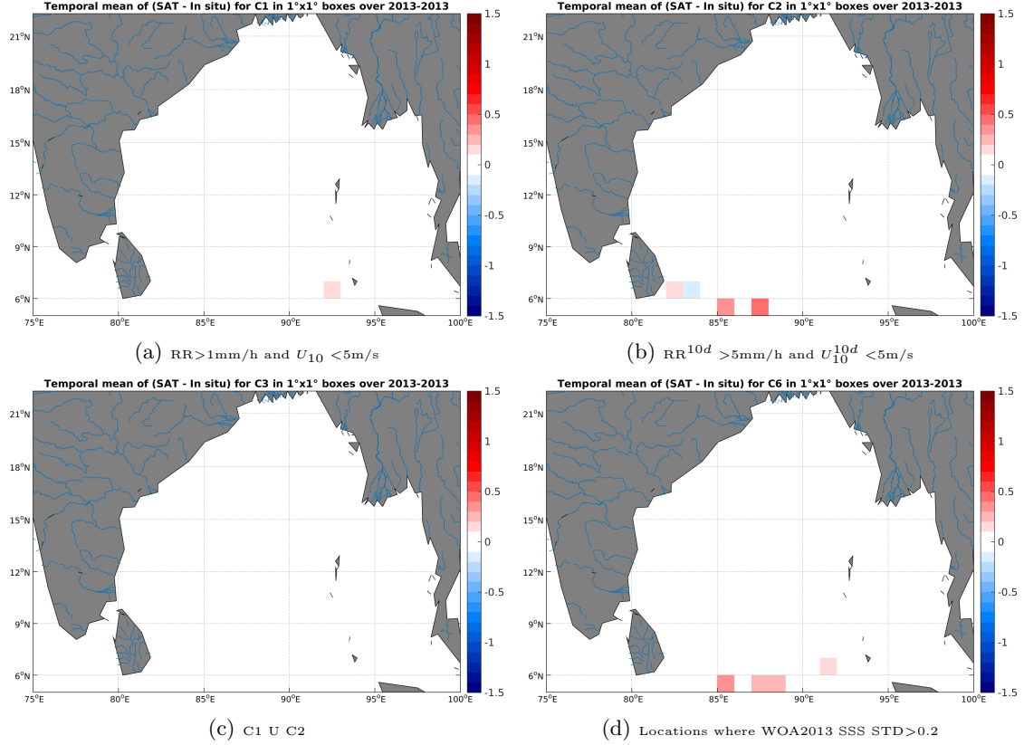
Figure 11: Temporal mean gridded over spatial boxes of size 1^\circ \times 1^\circ of \Delta SSS (Aquarius-L3-JPL-V4-MONTHLY - Surface drifters) for 4 different subdatasets corresponding to: RR > 1 mm/h and U_{10} < 5 m/s (a), RR 10d > 5 mm/h and U_{10}^{10d} < 5 m/s (b), C1 U C2 (c), Locations where WOA2013 SSS STD > 0.2 (d).
