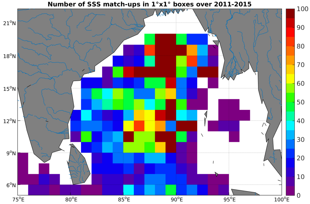
Figure 4: Number of SSS match-ups between Argo SSS and the Aquarius-L3-JPL-V4-MONTHLY SSS product for the Ganga and Brahmaputra river plumes Pi-MEP region over 1^\circ \times 1^\circ boxes and for the full satellite product period.
