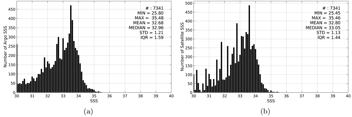
Figure 2: Histograms of SSS from Argo (a) and Aquarius-L3-JPL-V4-MONTHLY (b) considering all match-up pairs per bins of 0.1 over the Ganga and Brahmaputra river plumes Pi-MEP region and for the full satellite product period.
