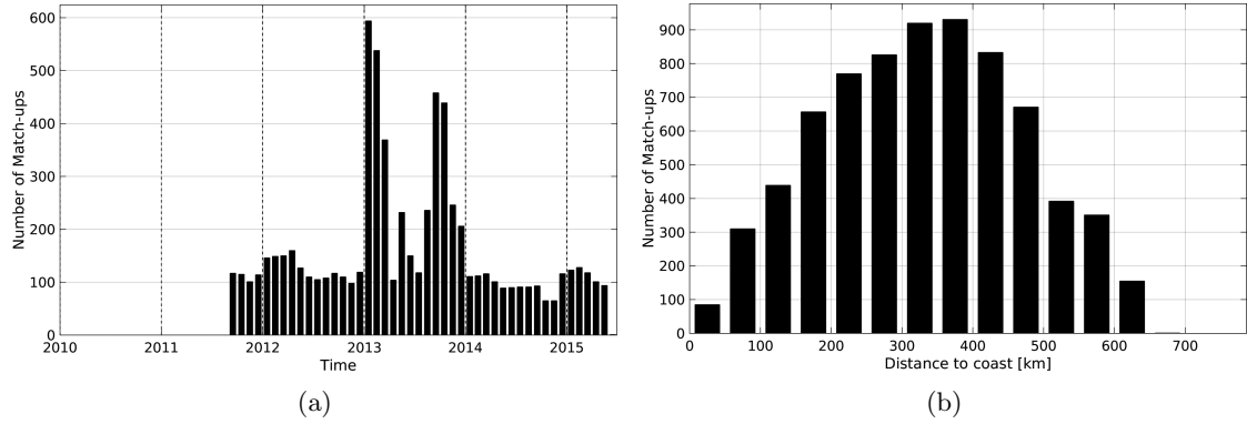
Figure 1: Number of match-ups between Argo and Aquarius-L3-JPL-V4-MONTHLY SSS as a function of time (a) and as function of the distance to coast (b) over the Ganga and Brahmaputra river plumes Pi-MEP region and for the full satellite product period.
