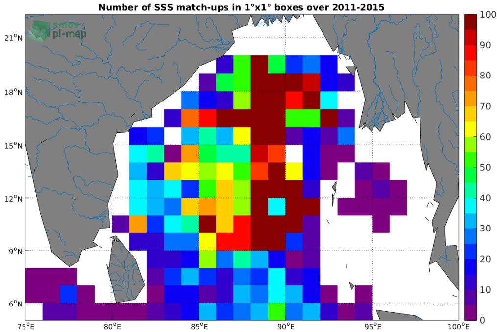
Figure 4: Number of SSS match-ups between Argo SSS and the Aquarius SSS L2-AVERAGED OR v5 (NASA-GSFC) SSS product for the Ganga and Brahmaputra river plumes Pi-MEP region over 1^\circ \times 1^\circ boxes and for the full satellite product period.
