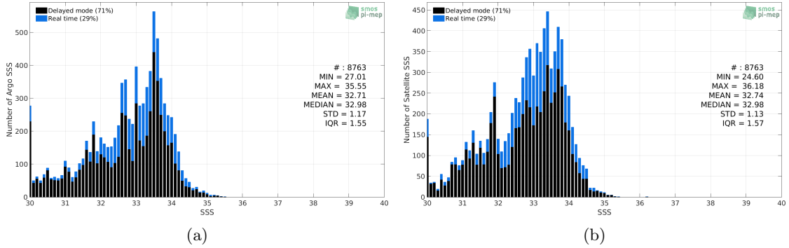
Figure 2: Histograms of SSS from Argo (a) and Aquarius SSS L2-AVERAGED OR v5 (NASA-GSFC) (b) considering all match-up pairs per bins of 0.1 over the Ganga and Brahmaputra river plumes Pi-MEP region and for the full satellite product period.
