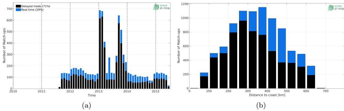
Figure 1: Number of match-ups between Argo and Aquarius SSS L2-AVERAGED OR v5 (NASA-GSFC) SSS as a function of time (a) and as function of the distance to coast (b) over the Ganga and Brahmaputra river plumes Pi-MEP region and for the full satellite product period.
