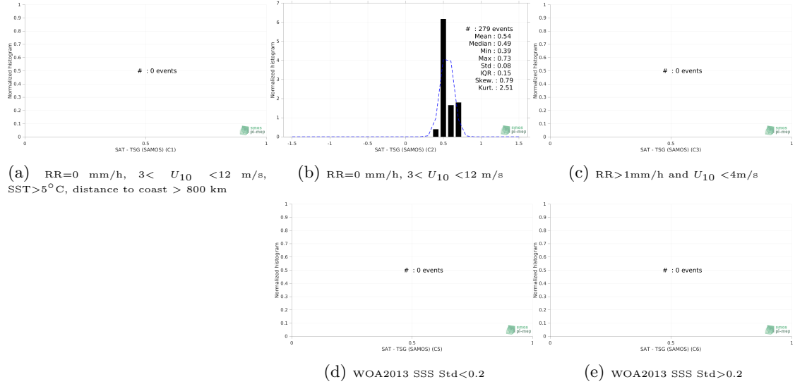
Figure 13: Normalized histogram of \Delta SSS (Aquarius SSS L2 OR v5 (NASA-GSFC) - TSG (SAMOS)) for 5 different subdatasets corresponding to: RR=0 mm/h, 3 < U_{10} < 12 m/s, SST > 5°C, distance to coast > 800 km (a), RR=0 mm/h, 3 < U_{10} < 12 m/s (b), RR > 1 mm/h and U_{10} < 4 m/s (c), WOA2013 SSS Std < 0.2 (d), WOA2013 SSS Std > 0.2 (e).
