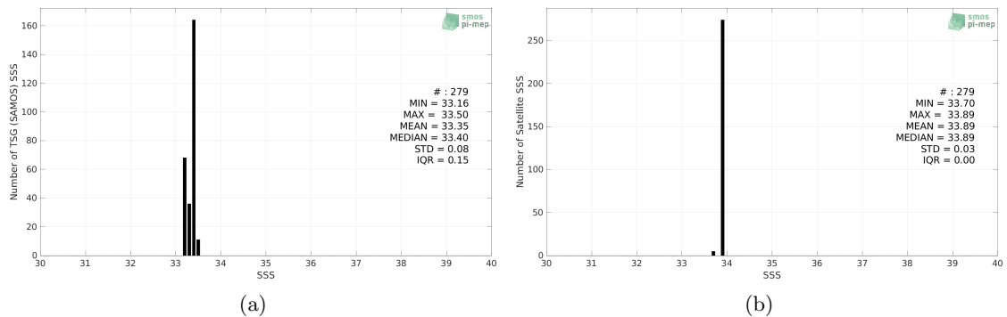
Figure 2: Histograms of SSS from TSG (SAMOS) (a) and Aquarius SSS L2 OR v5 (NASA-GSFC) (b) considering all match-up pairs per bins of 0.1 over the Ganga and Brahmaputra river plumes Pi-MEP region and for the full satellite product period.
