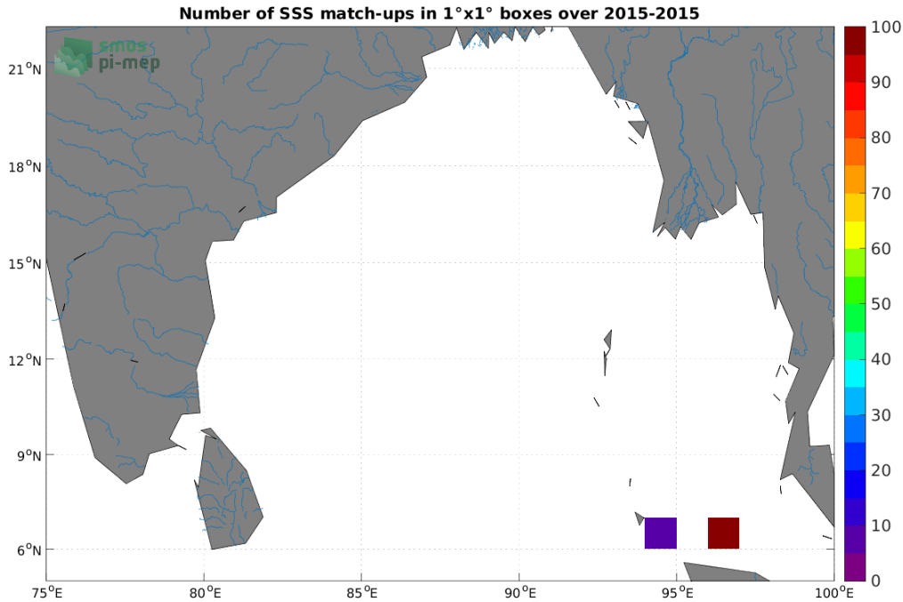
Figure 4: Number of SSS match-ups between TSG (SAMOS) SSS and the Aquarius SSS L2 OR v5 (NASA-GSFC) SSS product for the Ganga and Brahmaputra river plumes Pi-MEP region over 1°x1° boxes and for the full satellite product period.
