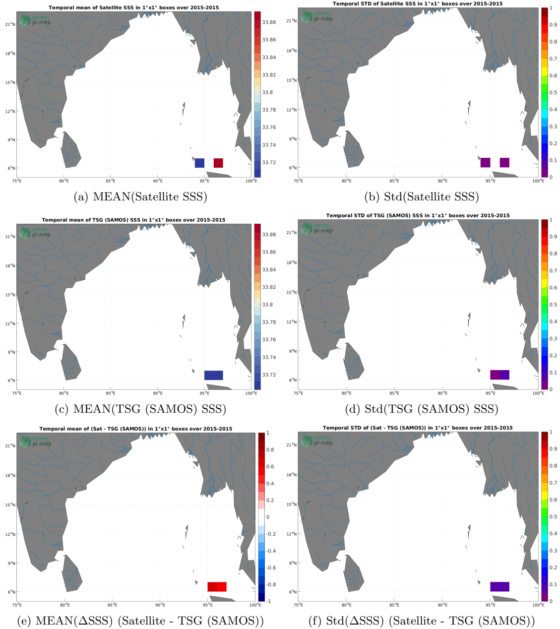
Figure 6: Temporal mean (left) and Std (right) of SSS from Aquarius SSS L2 OR v5 (NASA-GSFC) (top), TSG (SAMOS) (middle), and of \Delta SSS (Satellite - TSG (SAMOS)). Only match-up pairs are used to generate these maps.
