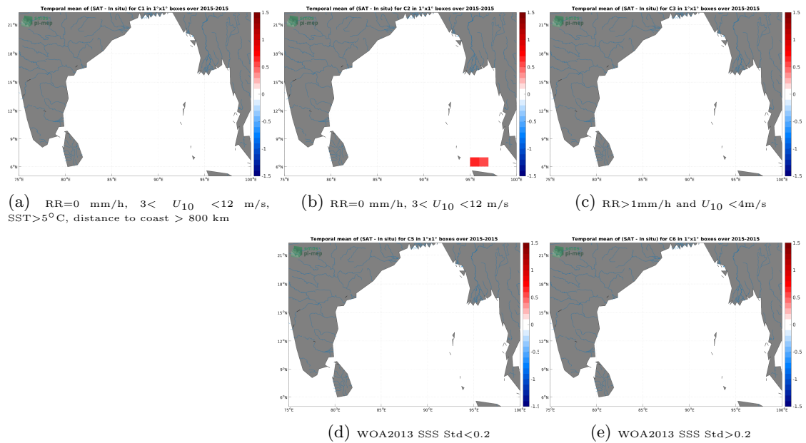
Figure 12: Temporal mean gridded over spatial boxes of size 1^\circ \times 1^\circ of \Delta SSS (Aquarius SSS L2 OR v5 (NASA-GSFC) - TSG (SAMOS)) for 5 different subdatasets corresponding to:RR=0 mm/h, 3 < U_{10} < 12 m/s, SST >5^\circ C, distance to coast > 800 km (a), RR=0 mm/h, 3 < U_{10} < 12 m/s (b), RR >1 mm/h and U_{10} < 4 m/s (c), WOA2013 SSS Std <0.2 (d), WOA2013 SSS Std >0.2 (e).
