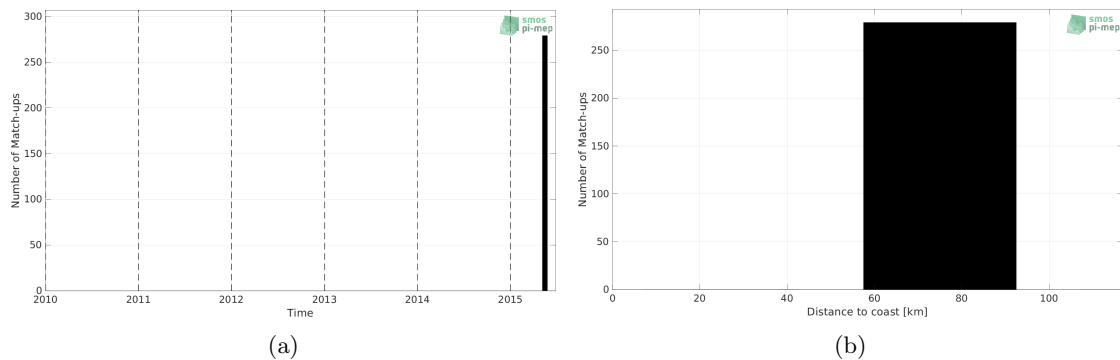
Figure 1: Number of match-ups between TSG (SAMOS) and Aquarius SSS L2 OR v5 (NASA-GSFC) SSS as a function of time (a) and as function of the distance to coast (b) over the Ganga and Brahmaputra river plumes Pi-MEP region and for the full satellite product period.
