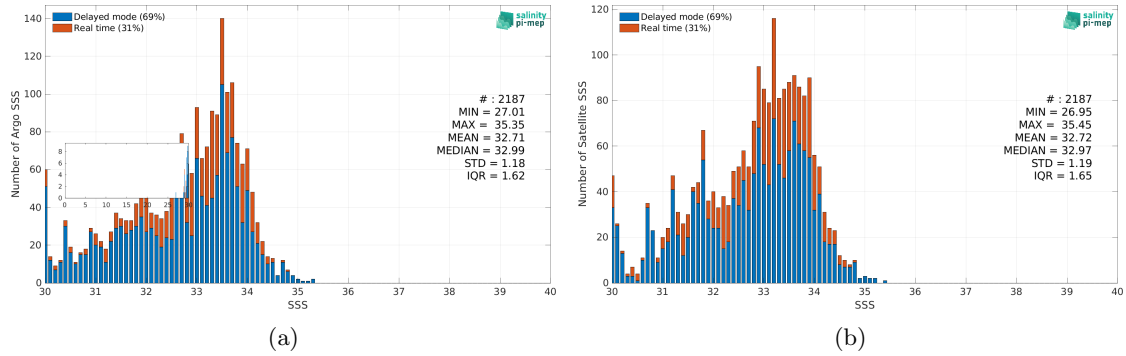
Figure 2: Histograms of SSS from Argo (a) and Aquarius SSS L2 OR v5 (NASA-GSFC) (b) considering all match-up pairs per bins of 0.1 over the Ganga and Brahmaputra river plumes Pi-MEP region and for the full satellite product period.
