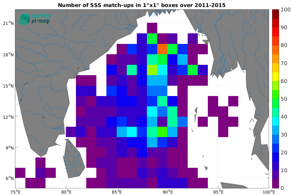
Figure 4: Number of SSS match-ups between Argo SSS and the Aquarius SSS L2 OR v5 (NASA-GSFC) SSS product for the Ganga and Brahmaputra river plumes Pi-MEP region over 1^\circ \times 1^\circ boxes and for the full satellite product period.
