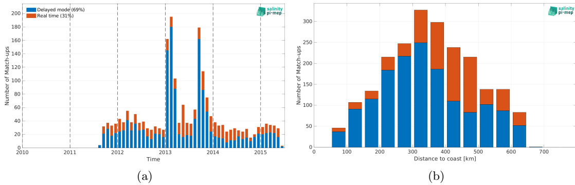
Figure 1: Number of match-ups between Argo and Aquarius SSS L2 OR v5 (NASA-GSFC) SSS as a function of time (a) and as function of the distance to coast (b) over the Ganga and Brahmaputra river plumes Pi-MEP region and for the full satellite product period.
