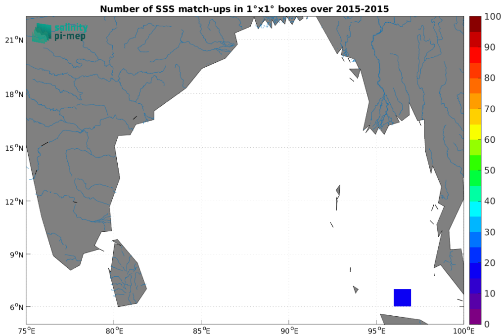
Figure 5: Number of SSS match-ups between TSG (SAMOS) SSS and the Aquarius SSS L2 CAP v5 (JPL) SSS product for the Ganga and Brahmaputra river plumes Pi-MEP region over 1^\circ \times 1^\circ boxes and for the full satellite product period.
