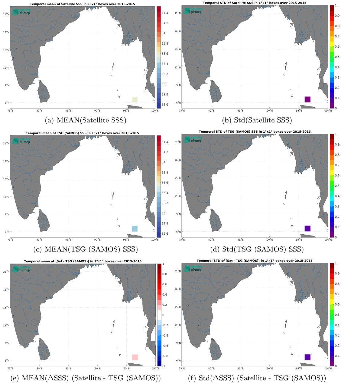
Figure 7: Temporal mean (left) and Std (right) of SSS from Aquarius SSS L2 CAP v5 (JPL) (top), TSG (SAMOS) (middle), and of \Delta SSS (Satellite - TSG (SAMOS)). Only match-up pairs are used to generate these maps.
