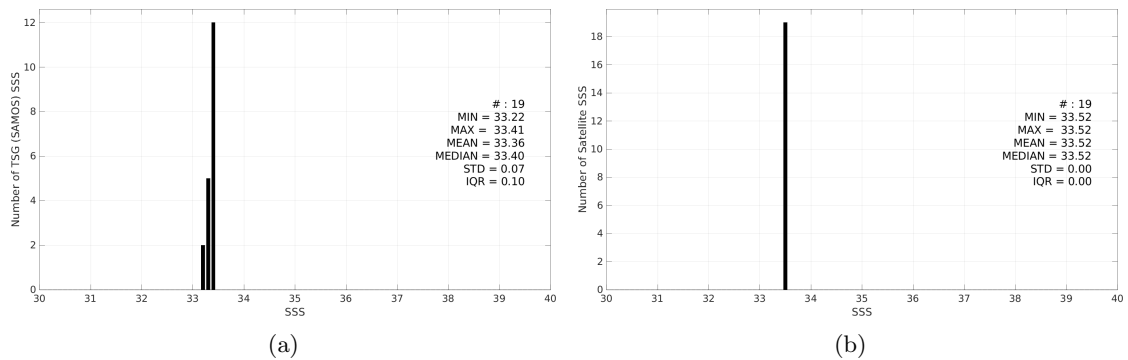
Figure 3: Histograms of SSS from TSG (SAMOS) (a) and Aquarius SSS L2 CAP v5 (JPL) (b) considering all match-up pairs per bins of 0.1 over the Ganga and Brahmaputra river plumes Pi-MEP region and for the full satellite product period.
