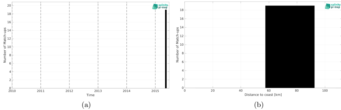
Figure 2: Number of match-ups between TSG (SAMOS) and Aquarius SSS L2 CAP v5 (JPL) SSS as a function of time (a) and as function of the distance to coast (b) over the Ganga and Brahmaputra river plumes Pi-MEP region and for the full satellite product period.
