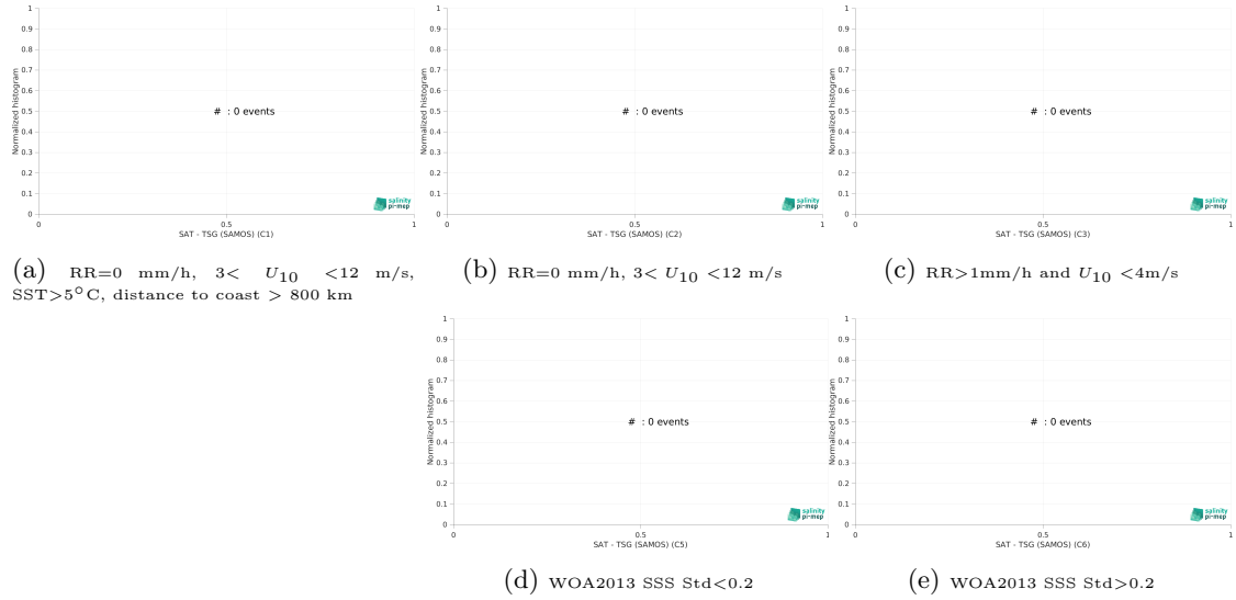
Figure 15: Normalized histogram of \Delta\text{SSS} (Aquarius SSS L2 CAP v5 (JPL) - TSG (SAMOS)) for 5 different subdatasets corresponding to: RR=0 mm/h, 3 < U_{10} < 12 m/s, SST > 5^\circ\text{C} , distance to coast > 800 km (a), RR=0 mm/h, 3 < U_{10} < 12 m/s (b), RR > 1 mm/h and U_{10} < 4 m/s (c), WOA2013 SSS Std < 0.2 (d), WOA2013 SSS Std > 0.2 (e).
