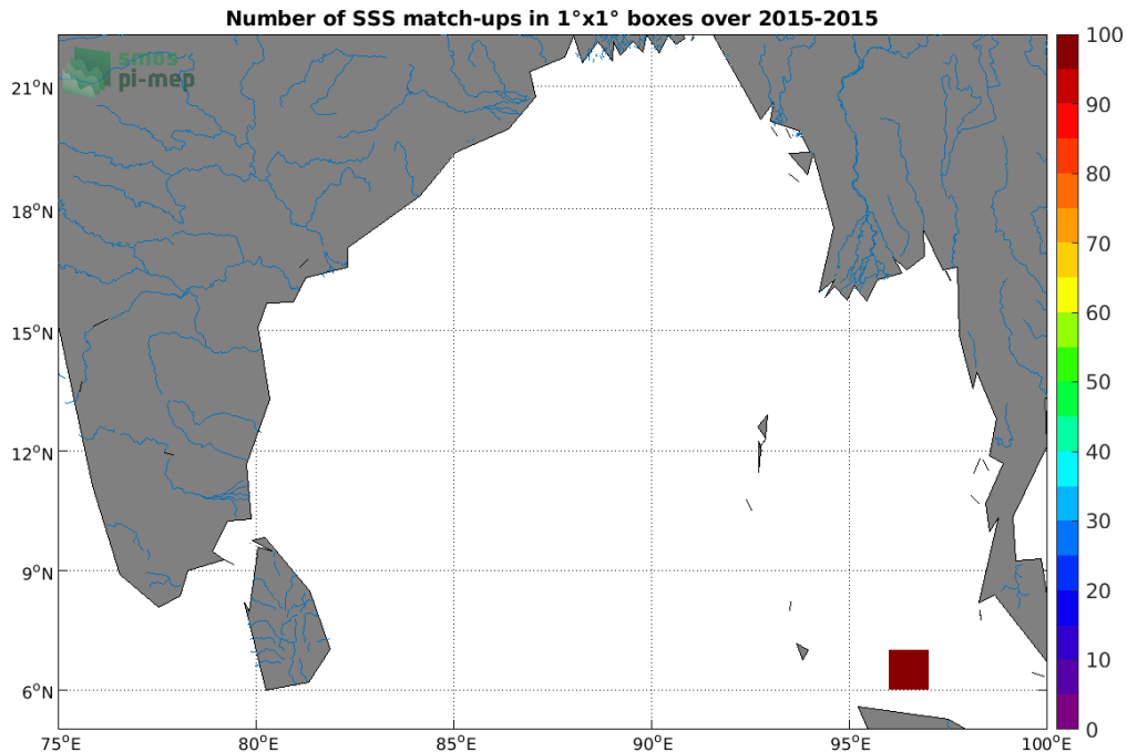
Figure 4: Number of SSS match-ups between TSG (SAMOS) SSS and the Aquarius SSS L2 CAP v5 (JPL) SSS product for the Ganga and Brahmaputra river plumes Pi-MEP region over 1^\circ \times 1^\circ boxes and for the full satellite product period.
