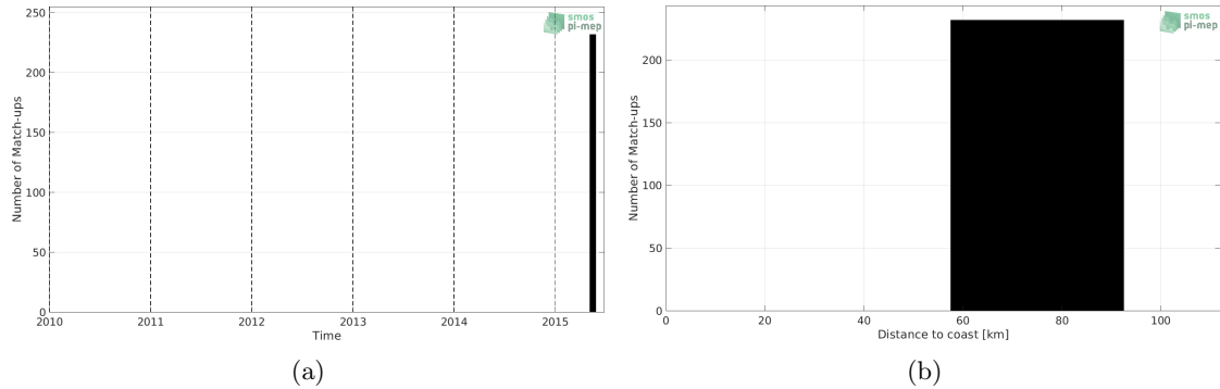
Figure 1: Number of match-ups between TSG (SAMOS) and Aquarius SSS L2 CAP v5 (JPL) SSS as a function of time (a) and as function of the distance to coast (b) over the Ganga and Brahmaputra river plumes Pi-MEP region and for the full satellite product period.
