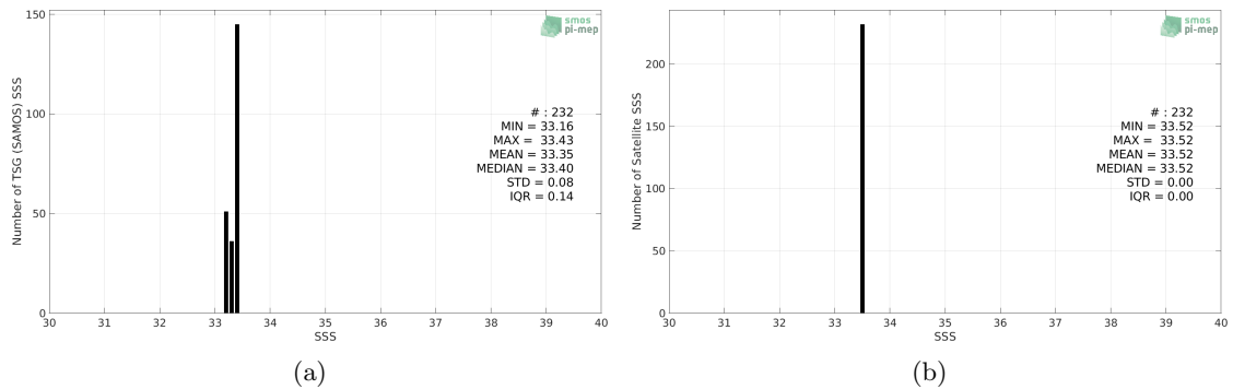
Figure 2: Histograms of SSS from TSG (SAMOS) (a) and Aquarius SSS L2 CAP v5 (JPL) (b) considering all match-up pairs per bins of 0.1 over the Ganga and Brahmaputra river plumes Pi-MEP region and for the full satellite product period.
