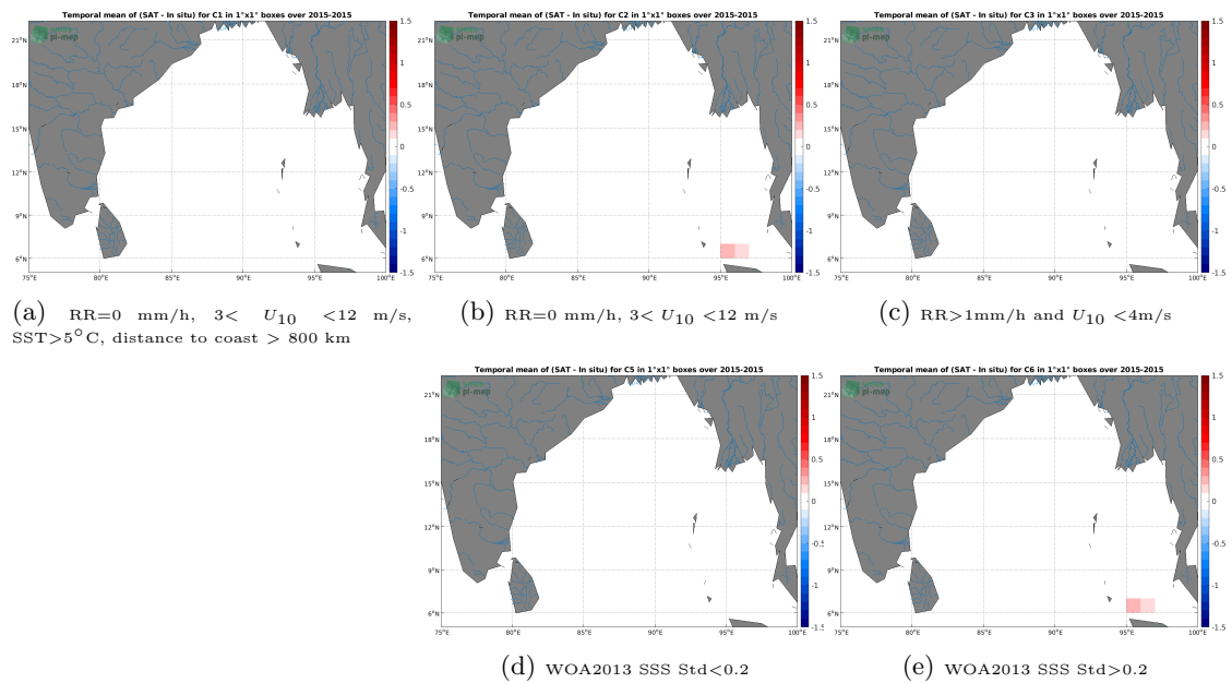
Figure 12: Temporal mean gridded over spatial boxes of size 1°x1° of \Delta SSS (Aquarius SSS L2 CAP v5 (JPL) - TSG (SAMOS)) for 5 different subdatasets corresponding to:RR=0 mm/h, 3 < U_{10} < 12 m/s, SST>5°C, distance to coast > 800 km (a), RR=0 mm/h, 3 < U_{10} < 12 m/s (b), RR>1mm/h and U_{10} < 4 m/s (c), WOA2013 SSS Std<0.2 (d), WOA2013 SSS Std>0.2 (e).
