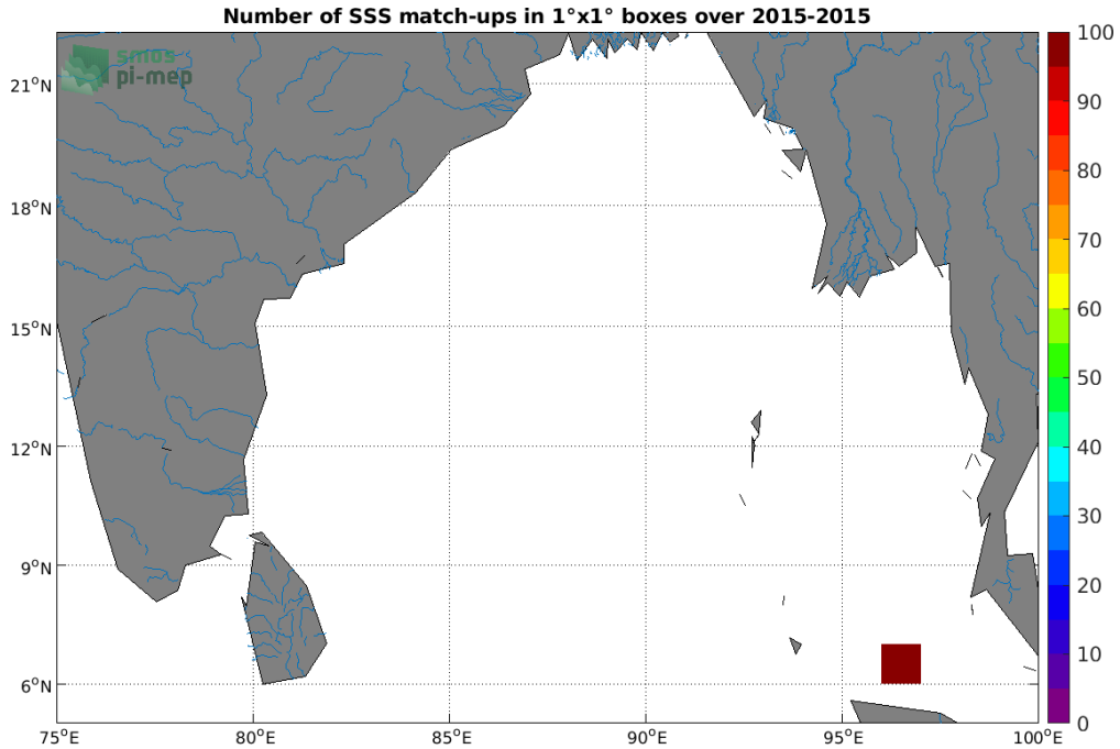
Figure 4: Number of SSS match-ups between TSG (SAMOS) SSS and the Aquarius SSS L2 CAP v5 (JPL) SSS product for the Ganga and Brahmaputra river plumes Pi-MEP region over 1°x1° boxes and for the full satellite product period.
