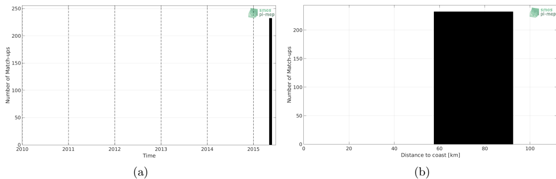
Figure 1: Number of match-ups between TSG-SAMOS and Aquarius-L2-JPL-V5 SSS as a function of time (a) and as function of the distance to coast (b) over the Ganga and Brahmaputra river plumes Pi-MEP region and for the full satellite product period.
