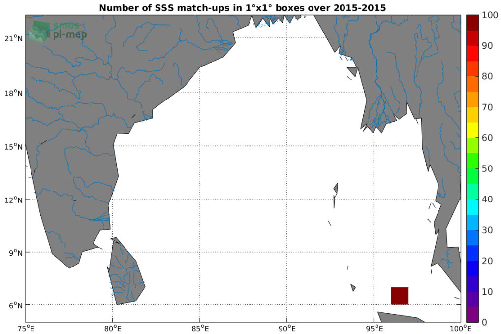
Figure 4: Number of SSS match-ups between TSG-SAMOS SSS and the Aquarius-L2-JPL-V5 SSS product for the Ganga and Brahmaputra river plumes Pi-MEP region over 1°x1° boxes and for the full satellite product period.
