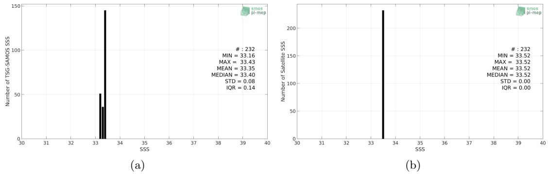
Figure 2: Histograms of SSS from TSG-SAMOS (a) and Aquarius-L2-JPL-V5 (b) considering all match-up pairs per bins of 0.1 over the Ganga and Brahmaputra river plumes Pi-MEP region and for the full satellite product period.
