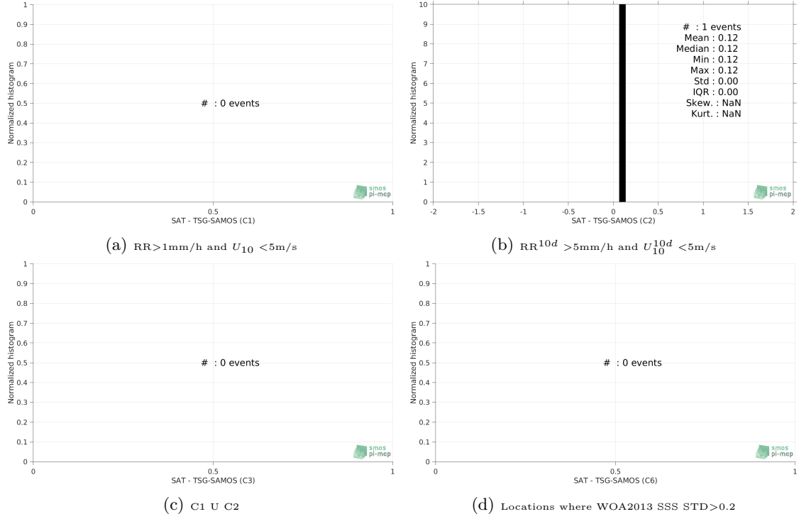
Figure 13: Normalized histogram of \Delta\text{SSS} (Aquarius-L2-JPL-V5 - TSG-SAMOS) for 6 different subdatasets corresponding to: RR > 1\text{mm/h} and U_{10} < 5\text{m/s} (a), RR^{10d} > 5\text{mm/h} and U_{10}^{10d} < 5\text{m/s} (b), C1 U C2 (c), Locations where WOA2013 SSS STD > 0.2 (d).
