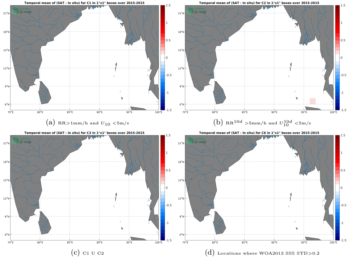
Figure 12: Temporal mean gridded over spatial boxes of size 1^\circ \times 1^\circ of \Delta SSS (Aquarius-L2-JPL-V5 - TSG-SAMOS) for 4 different subdatasets corresponding to: RR > 1mm/h and U_{10} < 5\text{m/s} (a), RR^{10d} > 5\text{mm/h} and U_{10}^{10d} < 5\text{m/s} (b), C1 U C2 (c), Locations where WOA2013 SSS STD > 0.2 (d).
