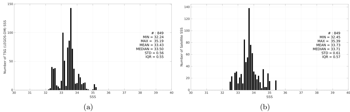
Figure 3: Histograms of SSS from TSG (LEGOS-DM) (a) and Aquarius SSS L2 CAP v5 (JPL) (b) considering all match-up pairs per bins of 0.1 over the Ganga and Brahmaputra river plumes Pi-MEP region and for the full satellite product period.
