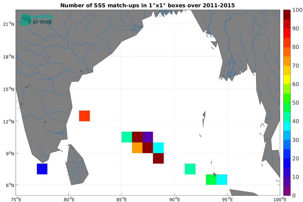
Figure 5: Number of SSS match-ups between TSG (LEGOS-DM) SSS and the Aquarius SSS L2 CAP v5 (JPL) SSS product for the Ganga and Brahmaputra river plumes Pi-MEP region over 1^\circ \times 1^\circ boxes and for the full satellite product period.
