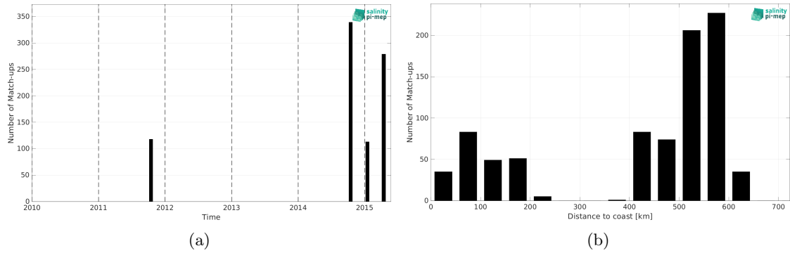
Figure 2: Number of match-ups between TSG (LEGOS-DM) and Aquarius SSS L2 CAP v5 (JPL) SSS as a function of time (a) and as function of the distance to coast (b) over the Ganga and Brahmaputra river plumes Pi-MEP region and for the full satellite product period.
