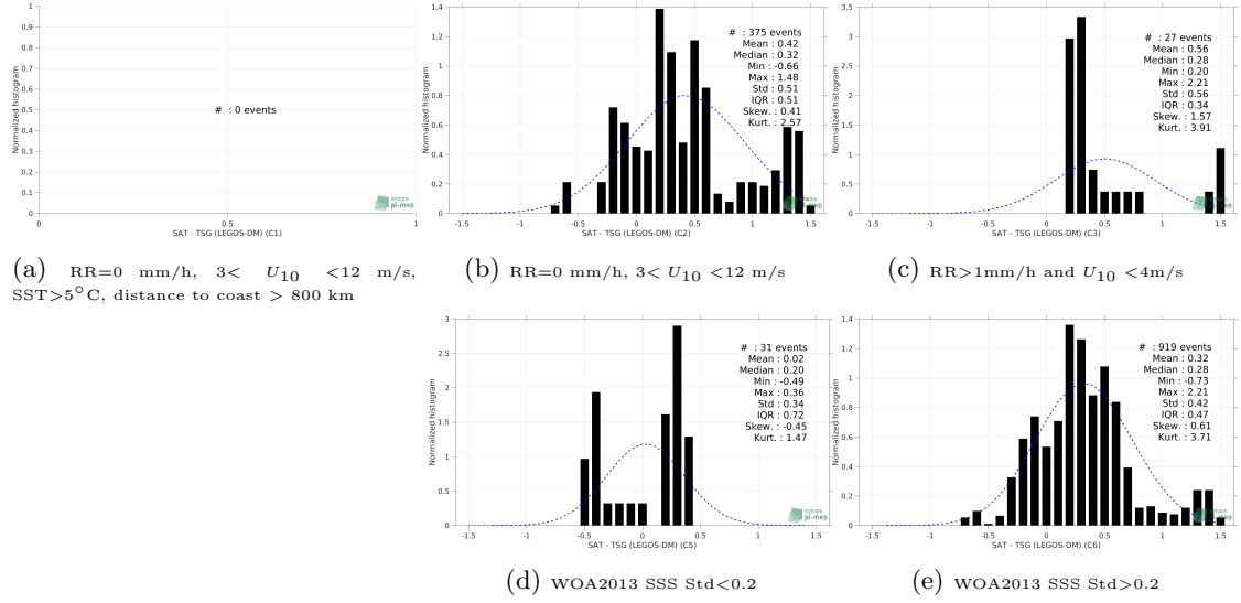
Figure 13: Normalized histogram of \Delta\text{SSS} (Aquarius SSS L2 CAP v5 (JPL) - TSG (LEGOS-DM)) for 5 different subdatasets corresponding to: RR=0 mm/h, 3 < U_{10} < 12 m/s, SST > 5^\circ\text{C} , distance to coast > 800 km (a), RR=0 mm/h, 3 < U_{10} < 12 m/s (b), RR > 1 mm/h and U_{10} < 4 m/s (c), WOA2013 SSS Std < 0.2 (d), WOA2013 SSS Std > 0.2 (e).
