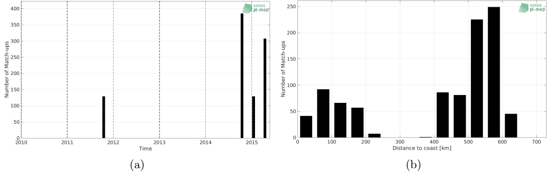
Figure 1: Number of match-ups between TSG (LEGOS-DM) and Aquarius SSS L2 CAP v5 (JPL) SSS as a function of time (a) and as function of the distance to coast (b) over the Ganga and Brahmaputra river plumes Pi-MEP region and for the full satellite product period.
