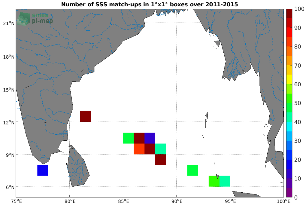
Figure 4: Number of SSS match-ups between TSG (LEGOS-DM) SSS and the Aquarius SSS L2 CAP v5 (JPL) SSS product for the Ganga and Brahmaputra river plumes Pi-MEP region over 1^\circ \times 1^\circ boxes and for the full satellite product period.
