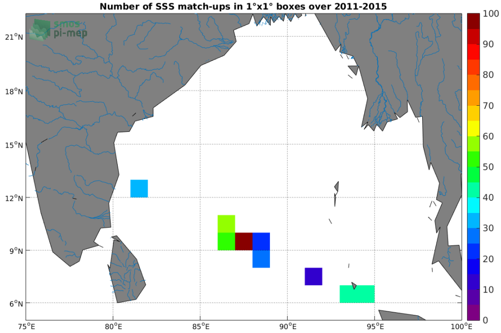
Figure 4: Number of SSS match-ups between TSG-LEGOS-DM SSS and the Aquarius-L2-JPL-V5 SSS product for the Ganga and Brahmaputra river plumes Pi-MEP region over 1^\circ \times 1^\circ boxes and for the full satellite product period.
