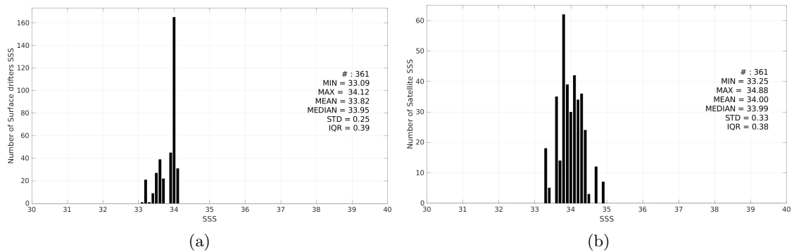
Figure 3: Histograms of SSS from Surface drifters (a) and Aquarius SSS L2 CAP v5 (JPL) (b) considering all match-up pairs per bins of 0.1 over the Ganga and Brahmaputra river plumes Pi-MEP region and for the full satellite product period.
