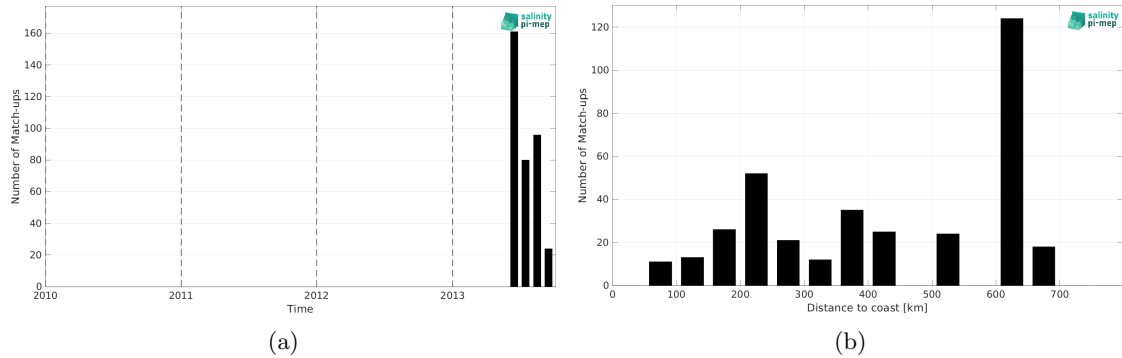
Figure 2: Number of match-ups between Surface drifters and Aquarius SSS L2 CAP v5 (JPL) SSS as a function of time (a) and as function of the distance to coast (b) over the Ganga and Brahmaputra river plumes Pi-MEP region and for the full satellite product period.
