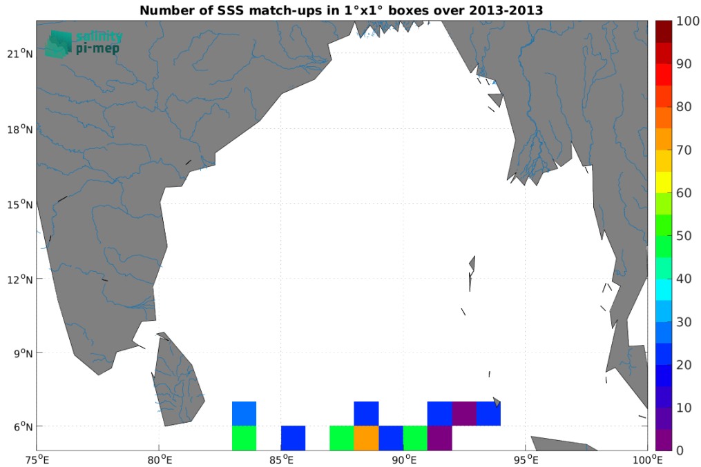
Figure 4: Number of SSS match-ups between Surface drifters SSS and the Aquarius SSS L2 CAP v5 (JPL) SSS product for the Ganga and Brahmaputra river plumes Pi-MEP region over 1^\circ \times 1^\circ boxes and for the full satellite product period.
