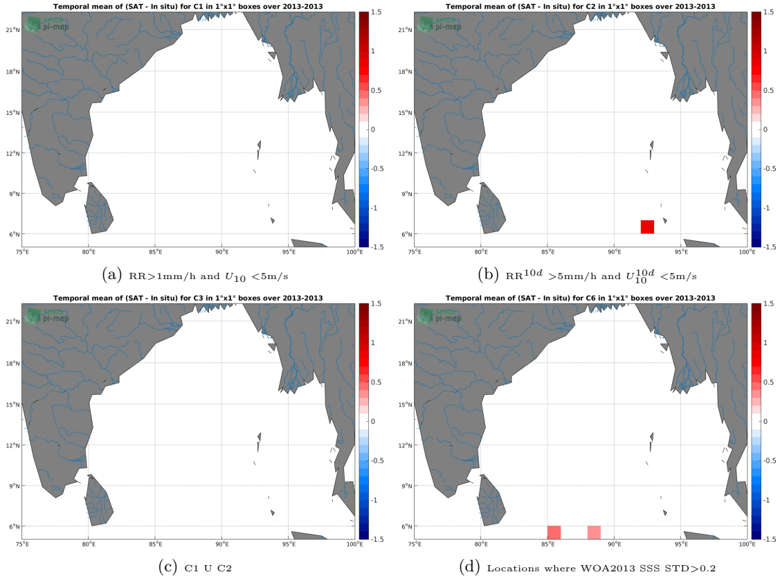
Figure 11: Temporal mean gridded over spatial boxes of size 1^\circ \times 1^\circ of \Delta SSS (Aquarius-L2-JPL-V5 - Surface drifters) for 4 different subdatasets corresponding to: RR > 1\text{mm/h} and U_{10} < 5\text{m/s} (a), RR^{10d} > 5\text{mm/h} and U_{10}^{10d} < 5\text{m/s} (b), C1 U C2 (c), Locations where WOA2013 SSS STD > 0.2 (d).
