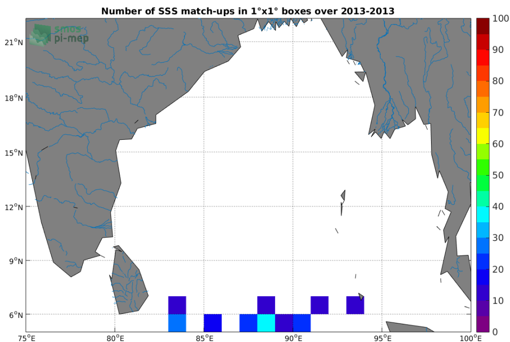
Figure 3: Number of SSS match-ups between Surface drifters SSS and the Aquarius-L2-JPL-V5 SSS product for the Ganga and Brahmaputra river plumes Pi-MEP region over 1°x1° boxes and for the full satellite product period.
