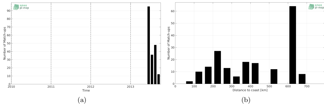
Figure 1: Number of match-ups between Surface drifters and Aquarius-L2-JPL-V5 SSS as a function of time (a) and as function of the distance to coast (b) over the Ganga and Brahmaputra river plumes Pi-MEP region and for the full satellite product period.
