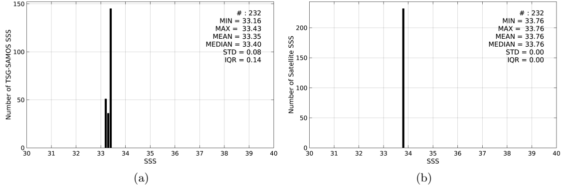
Figure 2: Histograms of SSS from TSG-SAMOS (a) and AQUARIUS-L2-JPL-V4 (b) considering all match-up pairs per bins of 0.1 over the Ganga and Brahmaputra river plumes Pi-MEP region and for the full satellite product period.
