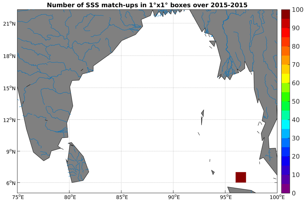
Figure 4: Number of SSS match-ups between TSG-SAMOS SSS and the AQUARIUS-L2-JPL-V4 SSS product for the Ganga and Brahmaputra river plumes Pi-MEP region over 1^\circ \times 1^\circ boxes and for the full satellite product period.
