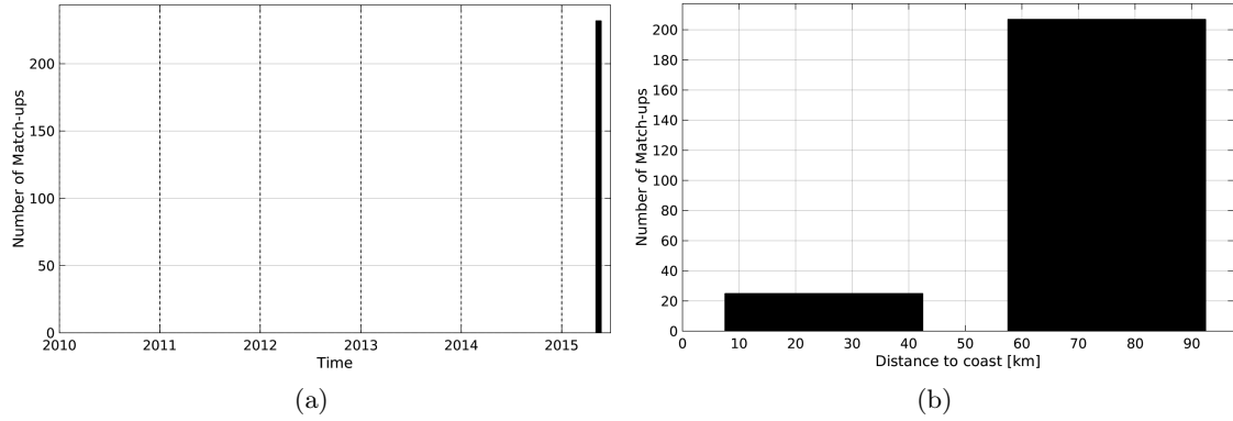
Figure 1: Number of match-ups between TSG-SAMOS and AQUARIUS-L2-JPL-V4 SSS as a function of time (a) and as function of the distance to coast (b) over the Ganga and Brahmaputra river plumes Pi-MEP region and for the full satellite product period.
