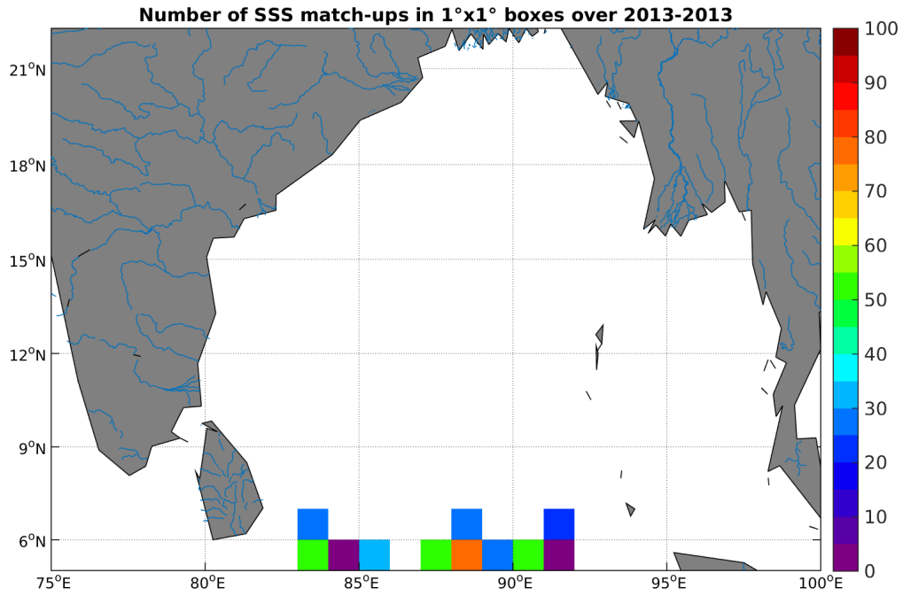
Figure 3: Number of SSS match-ups between Surface drifters SSS and the AQUARIUS-L2-JPL-V4 SSS product for the Ganga and Brahmaputra river plumes Pi-MEP region over 1°x1° boxes and for the full satellite product period.
