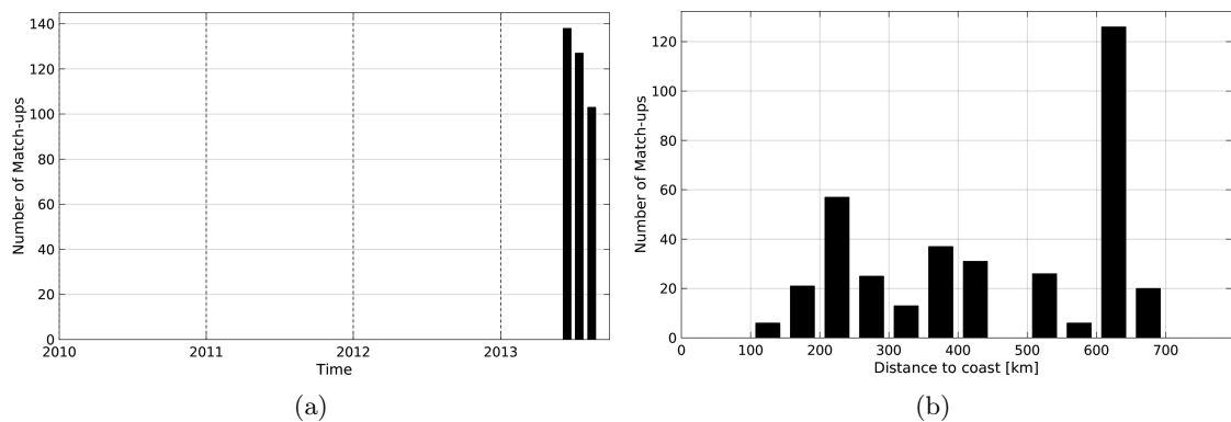
Figure 1: Number of match-ups between Surface drifters and AQUARIUS-L2-JPL-V4 SSS as a function of time (a) and as function of the distance to coast (b) over the Ganga and Brahmaputra river plumes Pi-MEP region and for the full satellite product period.
