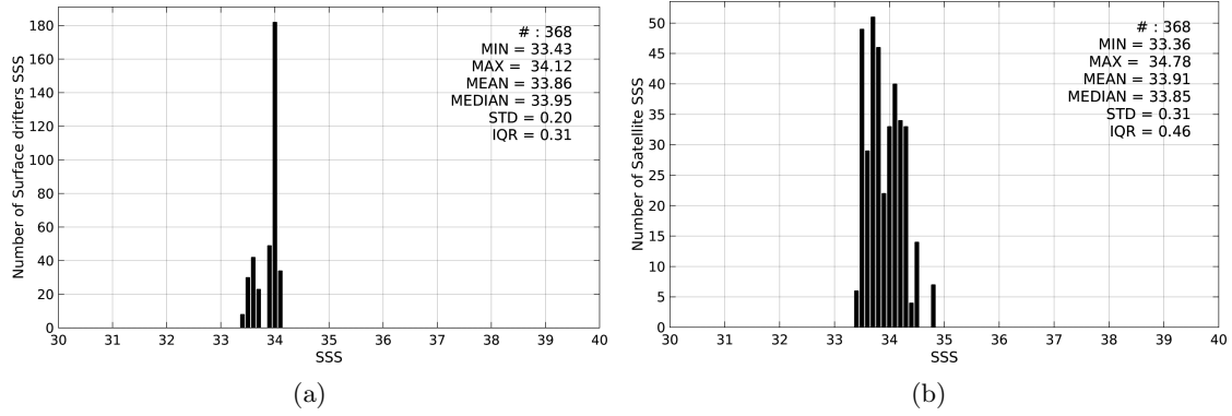
Figure 2: Histograms of SSS from Surface drifters (a) and AQUARIUS-L2-JPL-V4 (b) considering all match-up pairs per bins of 0.1 over the Ganga and Brahmaputra river plumes Pi-MEP region and for the full satellite product period.
