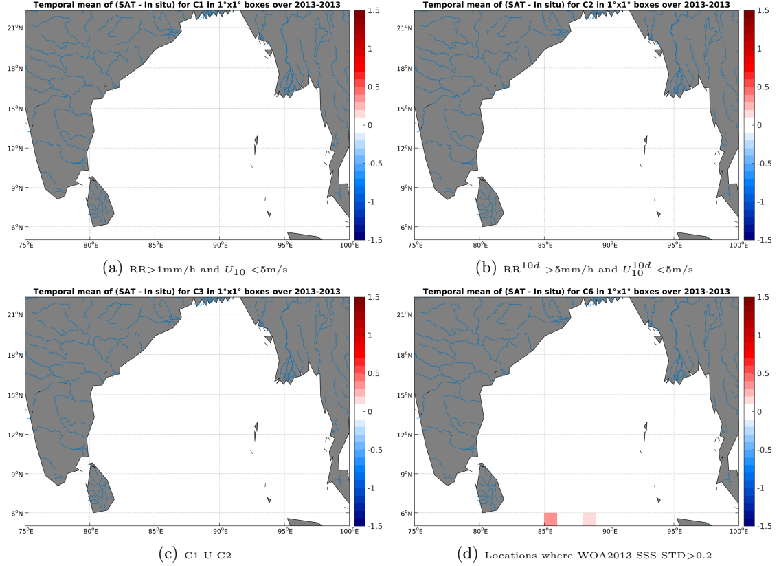
Figure 11: Temporal mean gridded over spatial boxes of size 1^\circ \times 1^\circ of \Delta SSS (AQUARIUS-L2-JPL-V4 - Surface drifters) for 4 different subdatasets corresponding to: RR > 1 mm/h and U_{10} < 5 m/s (a), RR 10d > 5 mm/h and U_{10}^{10d} < 5 m/s (b), C1 U C2 (c), Locations where WOA2013 SSS STD > 0.2 (d).
