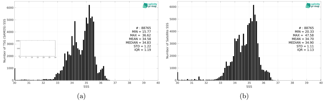
Figure 2: Histograms of SSS from TSG (SAMOS) (a) and SMOS and SMAP SSS L4 OI v1 - 7 Days (LOPS) (b) considering all match-up pairs per bins of 0.1 over the Equatorial Ocean 10N-10S Pi-MEP region and for the full satellite product period.
