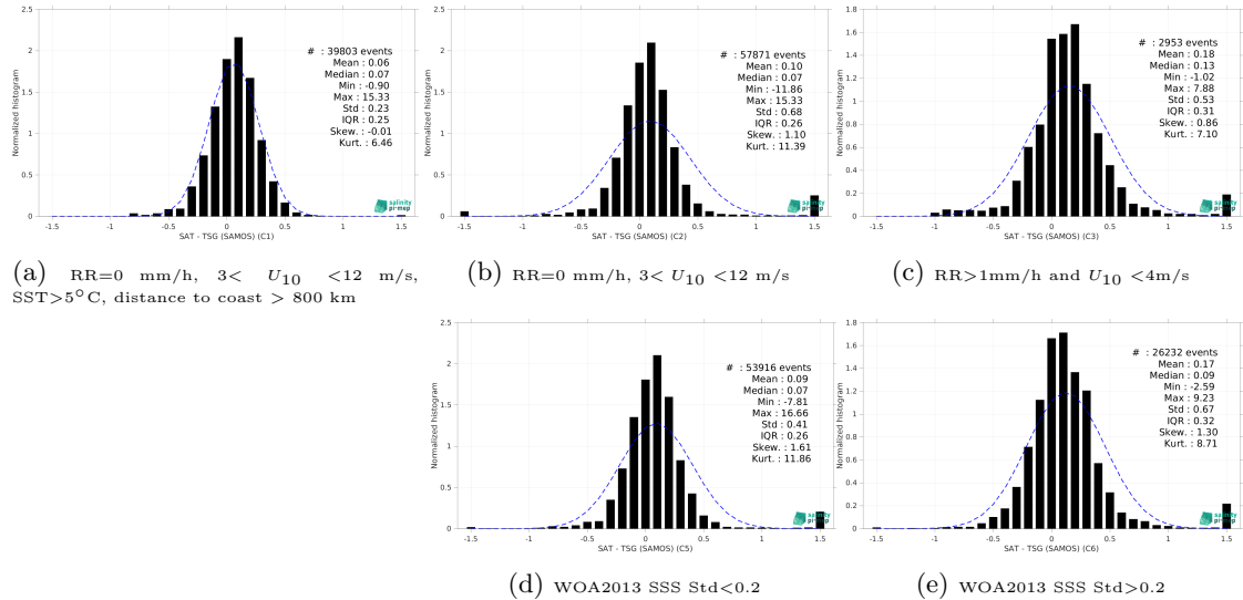
Figure 13: Normalized histogram of \Delta SSS (SMOS and SMAP SSS L4 OI v1 - 7 Days (LOPS) - TSG (SAMOS)) for 5 different subdatasets corresponding to: RR=0 mm/h, 3 < U_{10} < 12 m/s, SST >5^\circ\text{C} , distance to coast > 800 km (a), RR=0 mm/h, 3 < U_{10} < 12 m/s (b), RR >1 mm/h and U_{10} < 4 m/s (c), WOA2013 SSS Std <0.2 (d), WOA2013 SSS Std >0.2 (e).
