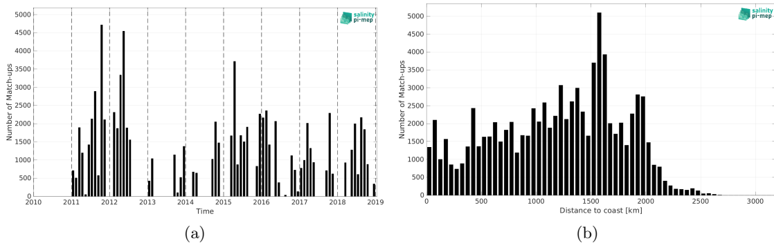
Figure 1: Number of match-ups between TSG (SAMOS) and SMOS and SMAP SSS L4 OI v1 - 7 Days (LOPS) SSS as a function of time (a) and as function of the distance to coast (b) over the Equatorial Ocean 10N-10S Pi-MEP region and for the full satellite product period.
