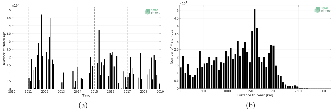
Figure 1: Number of match-ups between TSG (SAMOS) and SMOS and SMAP SSS L4 OI v1 - 7 Days (LOPS) SSS as a function of time (a) and as function of the distance to coast (b) over the Equatorial Ocean 10N-10S Pi-MEP region and for the full satellite product period.
