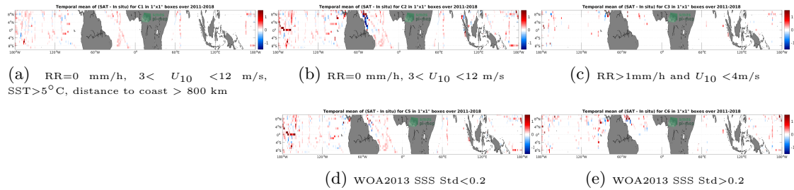
Figure 12: Temporal mean gridded over spatial boxes of size 1^\circ \times 1^\circ of \Delta SSS (SMOS and SMAP SSS L4 OI v1 - 7 Days (LOPS) - TSG (SAMOS)) for 5 different subdatasets corresponding to:RR=0 mm/h, 3 < U_{10} < 12 m/s, SST >5^\circ C, distance to coast > 800 km (a), RR=0 mm/h, 3 < U_{10} < 12 m/s (b), RR >1 mm/h and U_{10} < 4 m/s (c), WOA2013 SSS Std <0.2 (d), WOA2013 SSS Std >0.2 (e).
