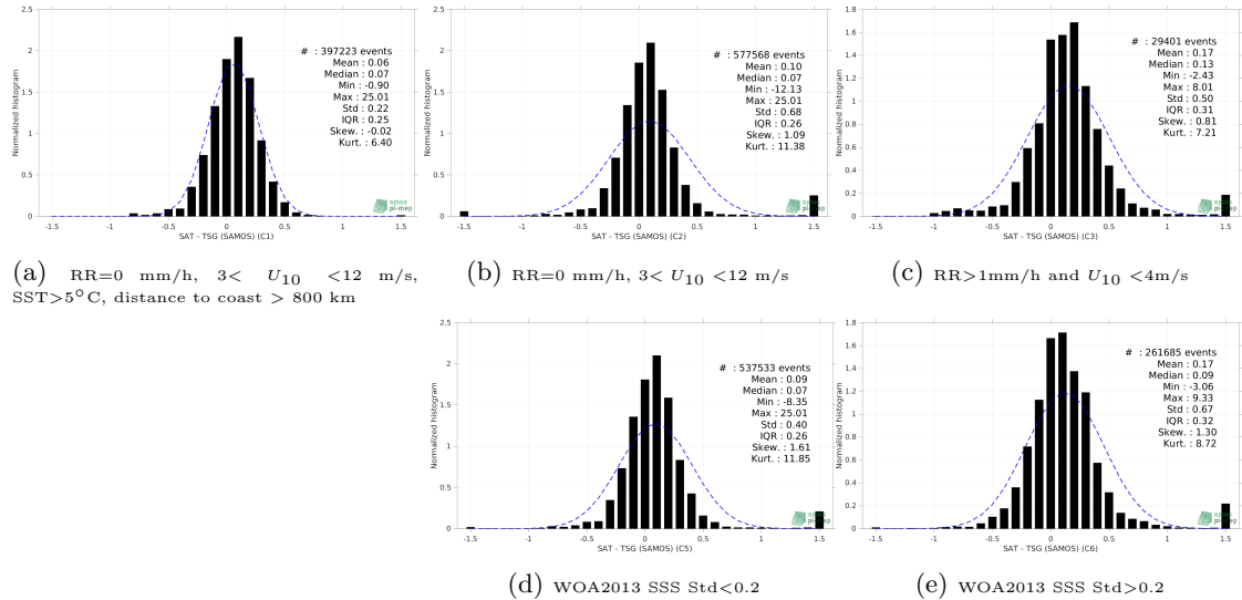
Figure 13: Normalized histogram of \Delta SSS (SMOS and SMAP SSS L4 OI v1 - 7 Days (LOPS) - TSG (SAMOS)) for 5 different subdatasets corresponding to: RR=0 mm/h, 3 < U_{10} < 12 m/s, SST >5^\circ C, distance to coast > 800 km (a), RR=0 mm/h, 3 < U_{10} < 12 m/s (b), RR >1 mm/h and U_{10} < 4 m/s (c), WOA2013 SSS Std <0.2 (d), WOA2013 SSS Std >0.2 (e).
