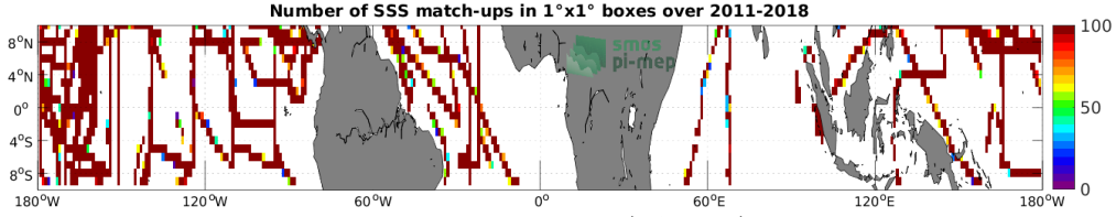
Figure 4: Number of SSS match-ups between TSG (SAMOS) SSS and the SMOS and SMAP SSS L4 OI v1 - 7 Days (LOPS) SSS product for the Equatorial Ocean 10N-10S Pi-MEP region over 1^\circ \times 1^\circ boxes and for the full satellite product period.
