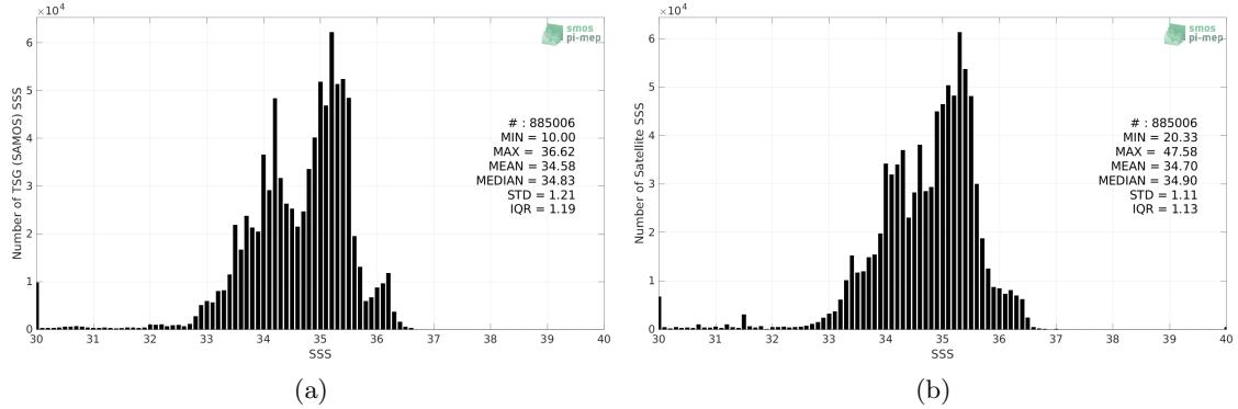
Figure 2: Histograms of SSS from TSG (SAMOS) (a) and SMOS and SMAP SSS L4 OI v1 - 7 Days (LOPS) (b) considering all match-up pairs per bins of 0.1 over the Equatorial Ocean 10N-10S Pi-MEP region and for the full satellite product period.
