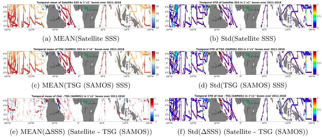
Figure 6: Temporal mean (left) and Std (right) of SSS from SMOS and SMAP SSS L4 OI v1 - 7 Days (LOPS) (top), TSG (SAMOS) (middle), and of \Delta SSS (Satellite - TSG (SAMOS)). Only match-up pairs are used to generate these maps.
