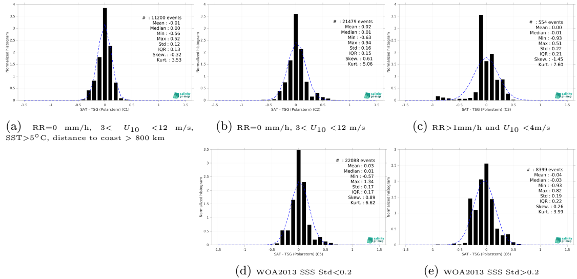
Figure 13: Normalized histogram of \Delta SSS (SMOS and SMAP SSS L4 OI v1 - 7 Days (LOPS) - TSG (Polarstern)) for 5 different subdatasets corresponding to: RR=0 mm/h, 3 < U_{10} < 12 m/s, SST >5^\circ C, distance to coast > 800 km (a), RR=0 mm/h, 3 < U_{10} < 12 m/s (b), RR >1 mm/h and U_{10} < 4 m/s (c), WOA2013 SSS Std <0.2 (d), WOA2013 SSS Std >0.2 (e).
