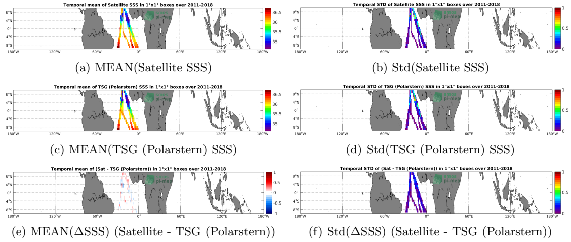
Figure 6: Temporal mean (left) and Std (right) of SSS from SMOS and SMAP SSS L4 OI v1 - 7 Days (LOPS) (top), TSG (Polarstern) (middle), and of \Delta SSS (Satellite - TSG (Polarstern)). Only match-up pairs are used to generate these maps.
