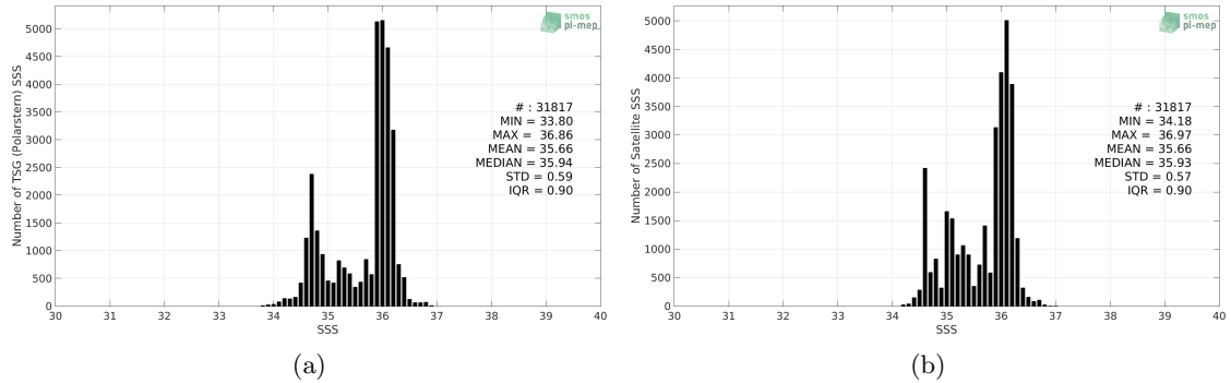
Figure 2: Histograms of SSS from TSG (Polarstern) (a) and SMOS and SMAP SSS L4 OI v1 - 7 Days (LOPS) (b) considering all match-up pairs per bins of 0.1 over the Equatorial Ocean 10N-10S Pi-MEP region and for the full satellite product period.
