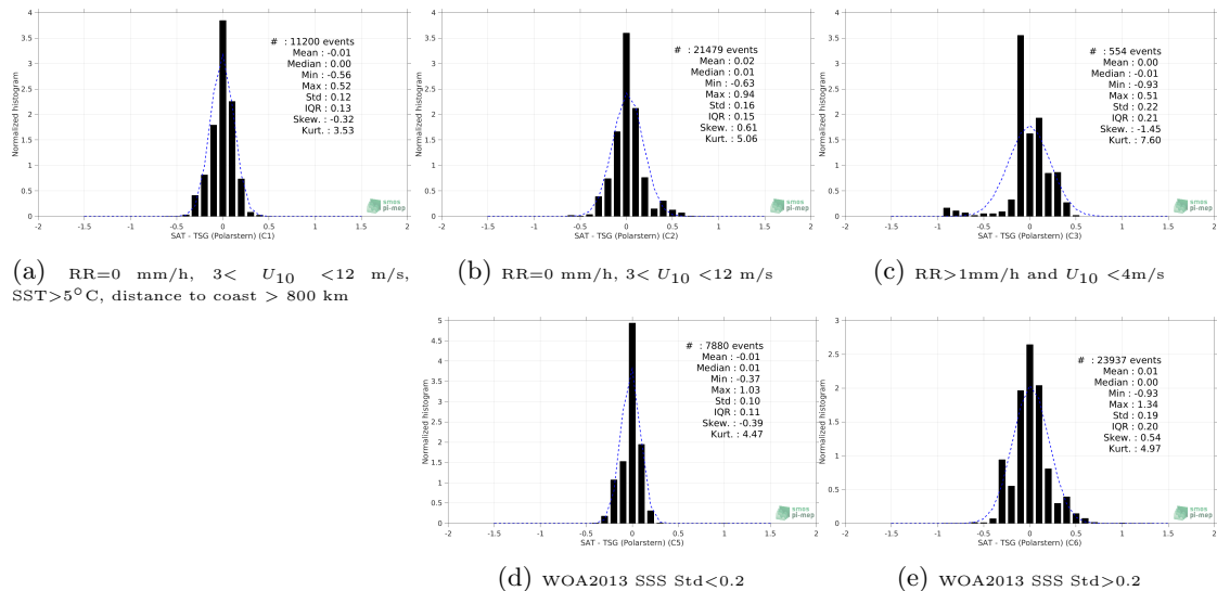
Figure 13: Normalized histogram of \Delta SSS (SMOS and SMAP SSS L4 OI v1 - 7 Days (LOPS) - TSG (Polarstern)) for 5 different subdatasets corresponding to: RR=0 mm/h, 3 < U_{10} < 12 m/s, SST >5^\circ\text{C} , distance to coast > 800 km (a), RR=0 mm/h, 3 < U_{10} < 12 m/s (b), RR >1 mm/h and U_{10} < 4 m/s (c), WOA2013 SSS Std <0.2 (d), WOA2013 SSS Std >0.2 (e).
