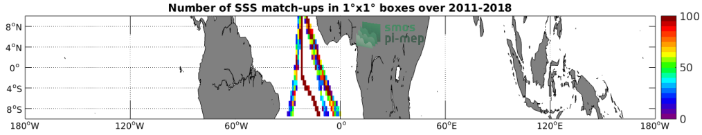
Figure 4: Number of SSS match-ups between TSG (Polarstern) SSS and the SMOS and SMAP SSS L4 OI v1 - 7 Days (LOPS) SSS product for the Equatorial Ocean 10N-10S Pi-MEP region over 1^\circ \times 1^\circ boxes and for the full satellite product period.
