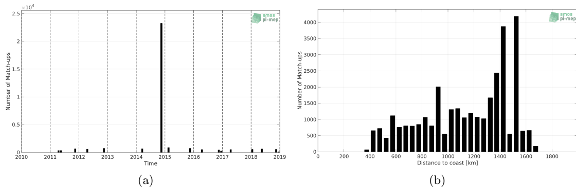
Figure 1: Number of match-ups between TSG (Polarstern) and SMOS and SMAP SSS L4 OI v1 - 7 Days (LOPS) SSS as a function of time (a) and as function of the distance to coast (b) over the Equatorial Ocean 10N-10S Pi-MEP region and for the full satellite product period.
