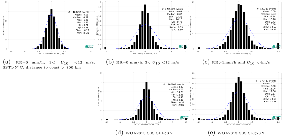
Figure 13: Normalized histogram of \Delta\text{SSS} (SMOS and SMAP SSS L4 OI v1 - 7 Days (LOPS) - TSG (LEGOS-DM)) for 5 different subdatasets corresponding to: RR=0 mm/h, 3 < U_{10} < 12 m/s, SST >5^\circ\text{C} , distance to coast > 800 km (a), RR=0 mm/h, 3 < U_{10} < 12 m/s (b), RR >1 mm/h and U_{10} < 4 m/s (c), WOA2013 SSS Std <0.2 (d), WOA2013 SSS Std >0.2 (e).
