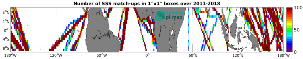
Figure 4: Number of SSS match-ups between TSG (LEGOS-DM) SSS and the SMOS and SMAP SSS L4 OI v1 - 7 Days (LOPS) SSS product for the Equatorial Ocean 10N-10S Pi-MEP region over 1^\circ \times 1^\circ boxes and for the full satellite product period.
