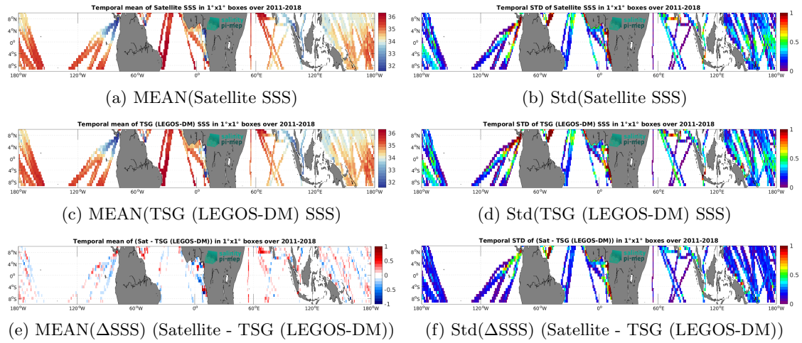
Figure 6: Temporal mean (left) and Std (right) of SSS from SMOS and SMAP SSS L4 OI v1 - 7 Days (LOPS) (top), TSG (LEGOS-DM) (middle), and of \Delta SSS (Satellite - TSG (LEGOS-DM)). Only match-up pairs are used to generate these maps.
