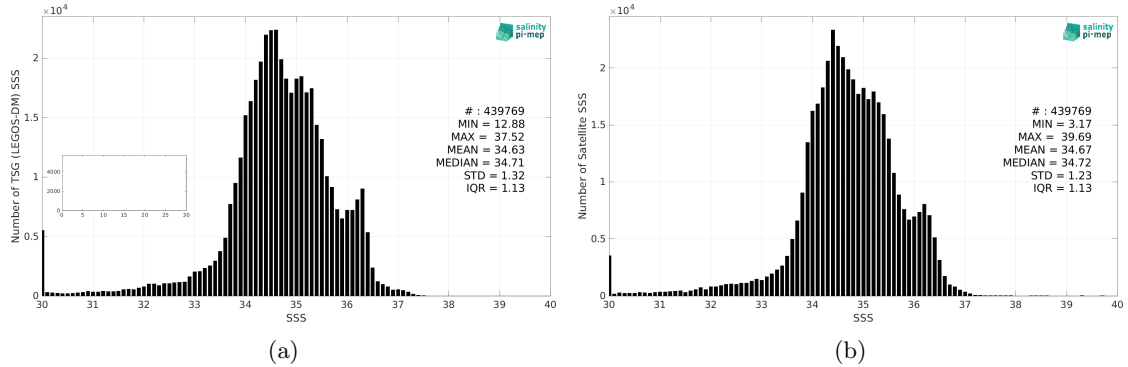
Figure 2: Histograms of SSS from TSG (LEGOS-DM) (a) and SMOS and SMAP SSS L4 OI v1 - 7 Days (LOPS) (b) considering all match-up pairs per bins of 0.1 over the Equatorial Ocean 10N-10S Pi-MEP region and for the full satellite product period.
