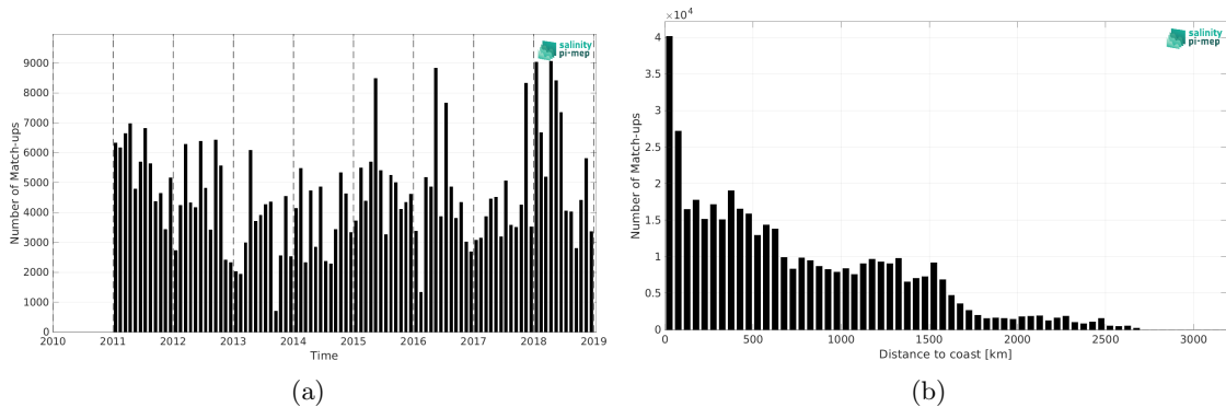
Figure 1: Number of match-ups between TSG (LEGOS-DM) and SMOS and SMAP SSS L4 OI v1 - 7 Days (LOPS) SSS as a function of time (a) and as function of the distance to coast (b) over the Equatorial Ocean 10N-10S Pi-MEP region and for the full satellite product period.
