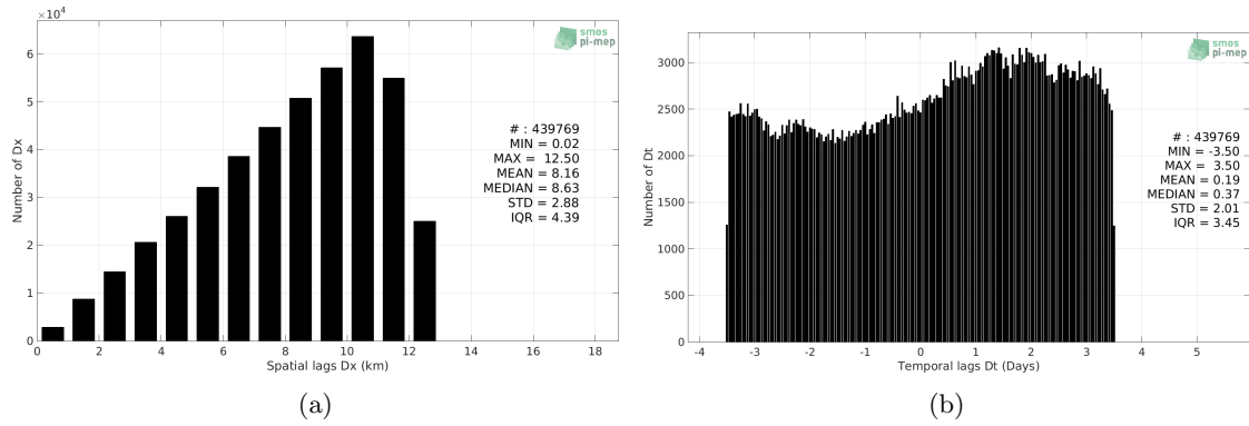
Figure 5: Histograms of the spatial (a) and temporal (b) lags between the location/time of the TSG (LEGOS-DM) measurement and the date of the corresponding SMOS and SMAP SSS L4 OI v1 - 7 Days (LOPS) SSS pixel.
