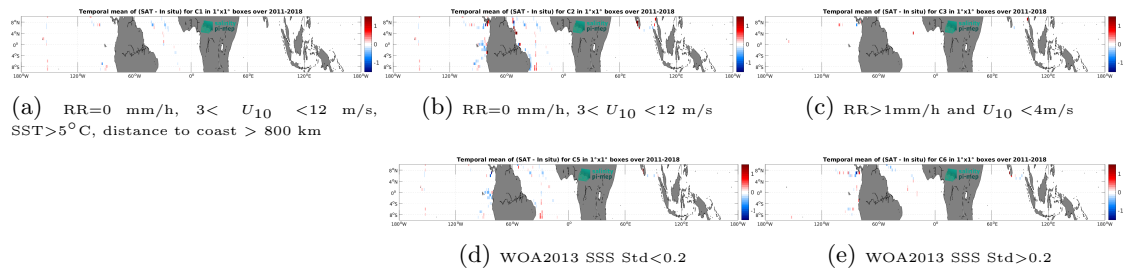
Figure 12: Temporal mean gridded over spatial boxes of size 1^{\circ}\times 1^{\circ} of \Delta SSS (SMOS and SMAP SSS L4 OI v1 - 7 Days (LOPS) - TSG (GOSUD-Sailing-ship)) for 5 different subdatasets corresponding to:RR=0 mm/h, 3 < U_{10} < 12 m/s, SST >5^{\circ}\text{C} , distance to coast > 800 km (a), RR=0 mm/h, 3 < U_{10} < 12 m/s (b), RR >1 mm/h and U_{10} < 4 m/s (c), WOA2013 SSS Std <0.2 (d), WOA2013 SSS Std >0.2 (e).
