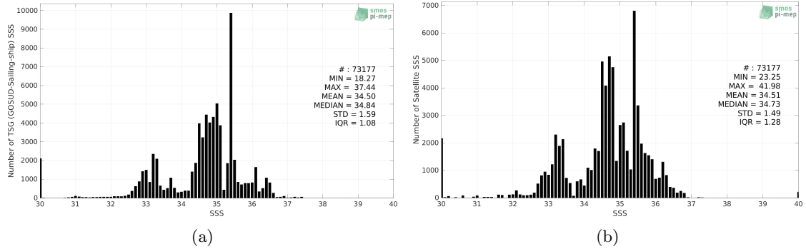
Figure 2: Histograms of SSS from TSG (GOSUD-Sailing-ship) (a) and SMOS and SMAP SSS L4 OI v1 - 7 Days (LOPS) (b) considering all match-up pairs per bins of 0.1 over the Equatorial Ocean 10N-10S Pi-MEP region and for the full satellite product period.
