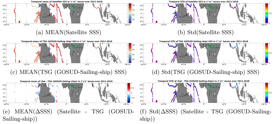
Figure 6: Temporal mean (left) and Std (right) of SSS from SMOS and SMAP SSS L4 OI v1 - 7 Days (LOPS) (top), TSG (GOSUD-Sailing-ship) (middle), and of \Delta SSS (Satellite - TSG (GOSUD-Sailing-ship)). Only match-up pairs are used to generate these maps.
