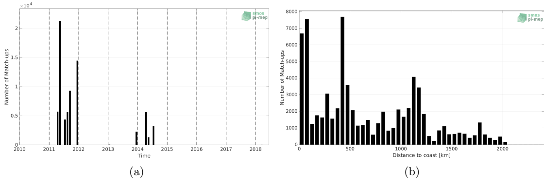
Figure 1: Number of match-ups between TSG (GOSUD-Sailing-ship) and SMOS and SMAP SSS L4 OI v1 - 7 Days (LOPS) SSS as a function of time (a) and as function of the distance to coast (b) over the Equatorial Ocean 10N-10S Pi-MEP region and for the full satellite product period.
