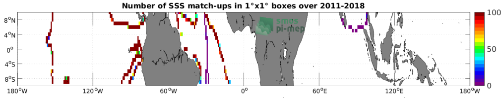
Figure 4: Number of SSS match-ups between TSG (GOSUD-Sailing-ship) SSS and the SMOS and SMAP SSS L4 OI v1 - 7 Days (LOPS) SSS product for the Equatorial Ocean 10N-10S Pi-MEP region over 1^\circ \times 1^\circ boxes and for the full satellite product period.
